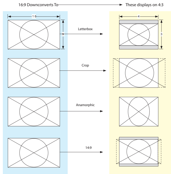
Figure 34. Down-Convert Illustrations
