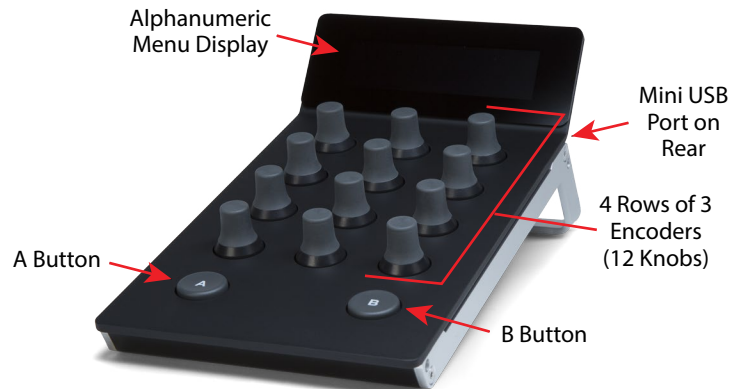
Figure 45. Tangent Element Kb Panel
