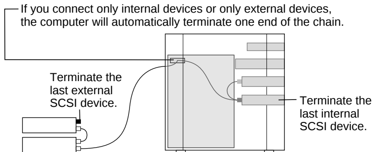
Narrow SCSI-1 Bus Termination
