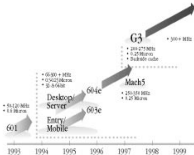
PowerPC Processor Roadmap
