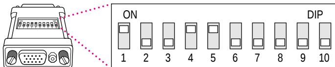
Dip Switch Settings for Video Terminator
