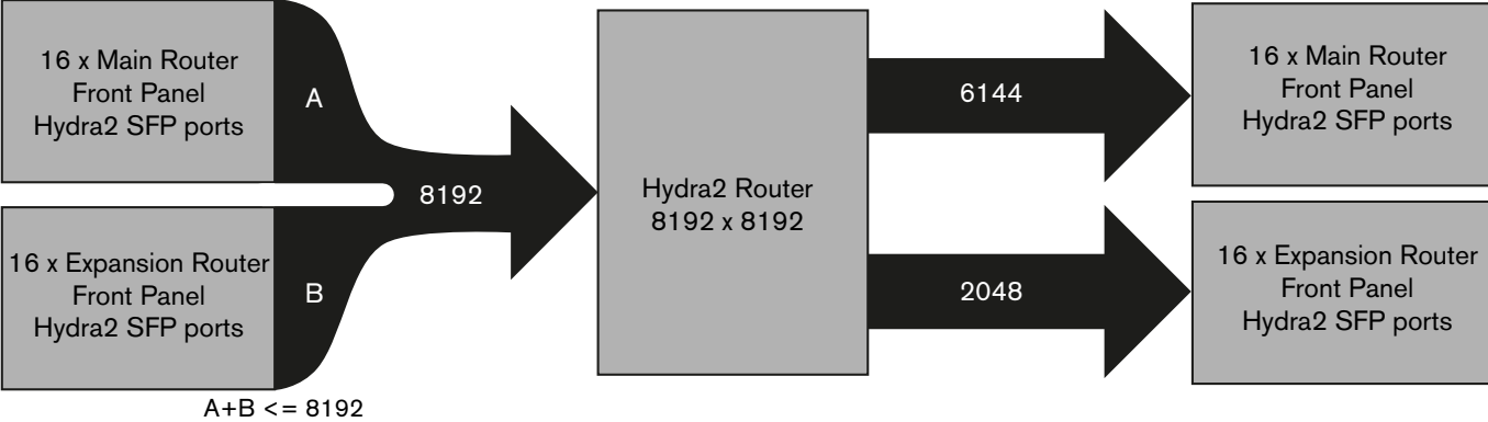
8U Router Core with Expansion fitted (no DSP)
