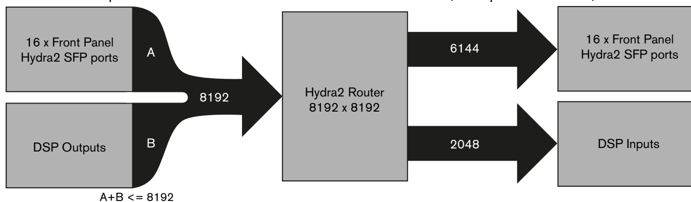
Apollo/Artemis-Shine/Artemis-Beam Console Core (no Expansion Router)
