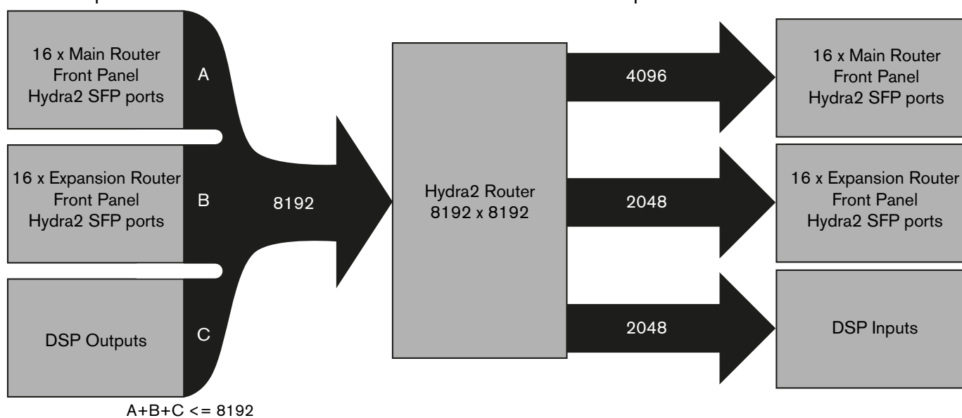
Apollo/Artemis-Shine/Artemis-Beam Console Core with Expansion Router card fitted.
