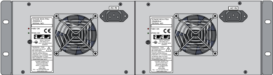
FIGURE 2 - STAGEBOX REAR
