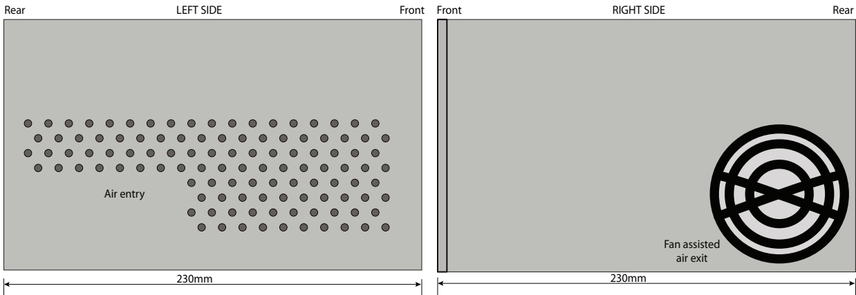
FIGURE 6 - AE5743 - SIDE VIEWS
