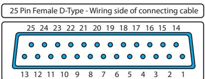
FIGURE 3 - GPO CONNECTING CABLE PIN ASSIGNMENTS
