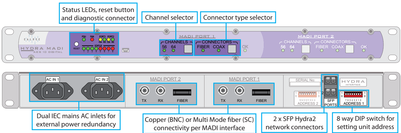
FIGURE 2 - JM5736 - DUAL MADI INTERFACE
