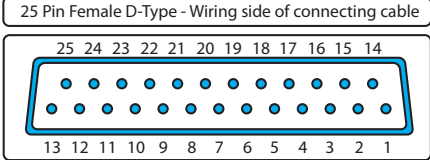
FIGURE 3 - OUTPUT WIRING
