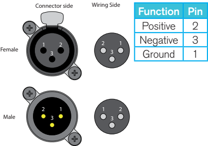
FIGURE 4 - XLR CONNECTORS
