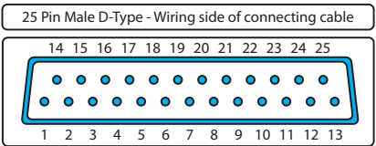
FIGURE 2 - GPI CONNECTING CABLE PIN ASSIGNMENTS
