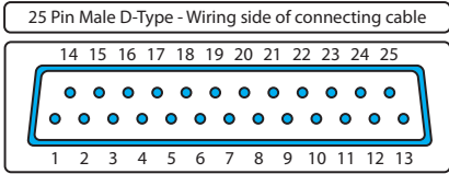
FIGURE 2 - INPUT WIRING
