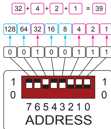
FIGURE 2 - ADDRESS EXAMPLE
