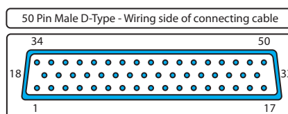
FIGURE 2 - GP INPUT PINS
