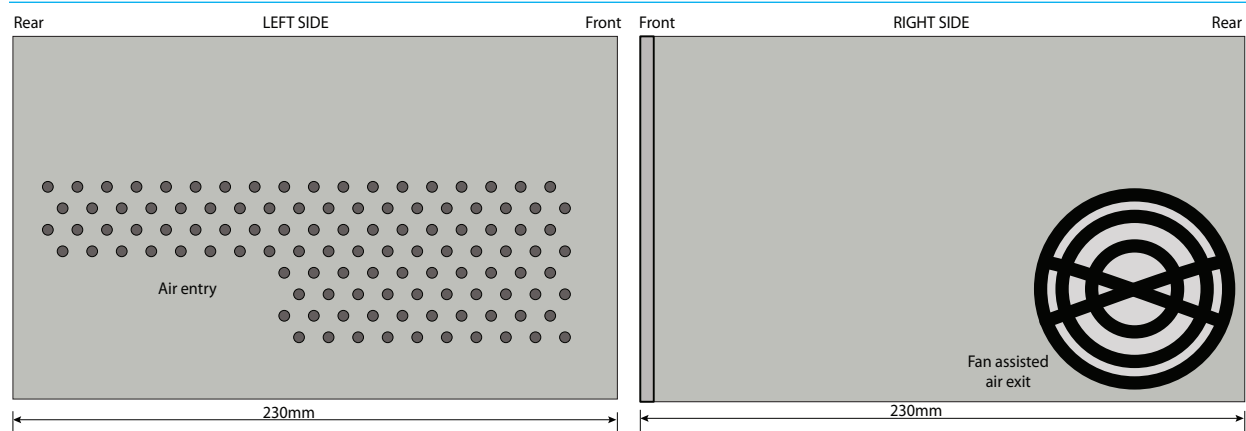
FIGURE 4 - JB5783 - SIDE VIEWS
