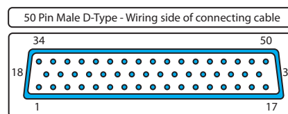
FIGURE 3 - GP INPUT PINS
