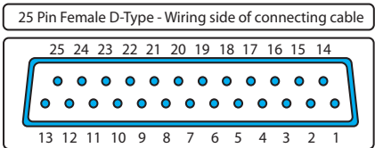
FIGURE 2 - METADATA WIRING
