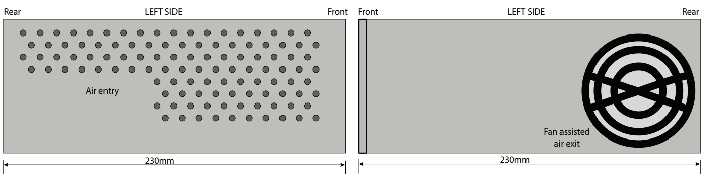
FIGURE 4 - JB5606 - SIDE VIEWS
