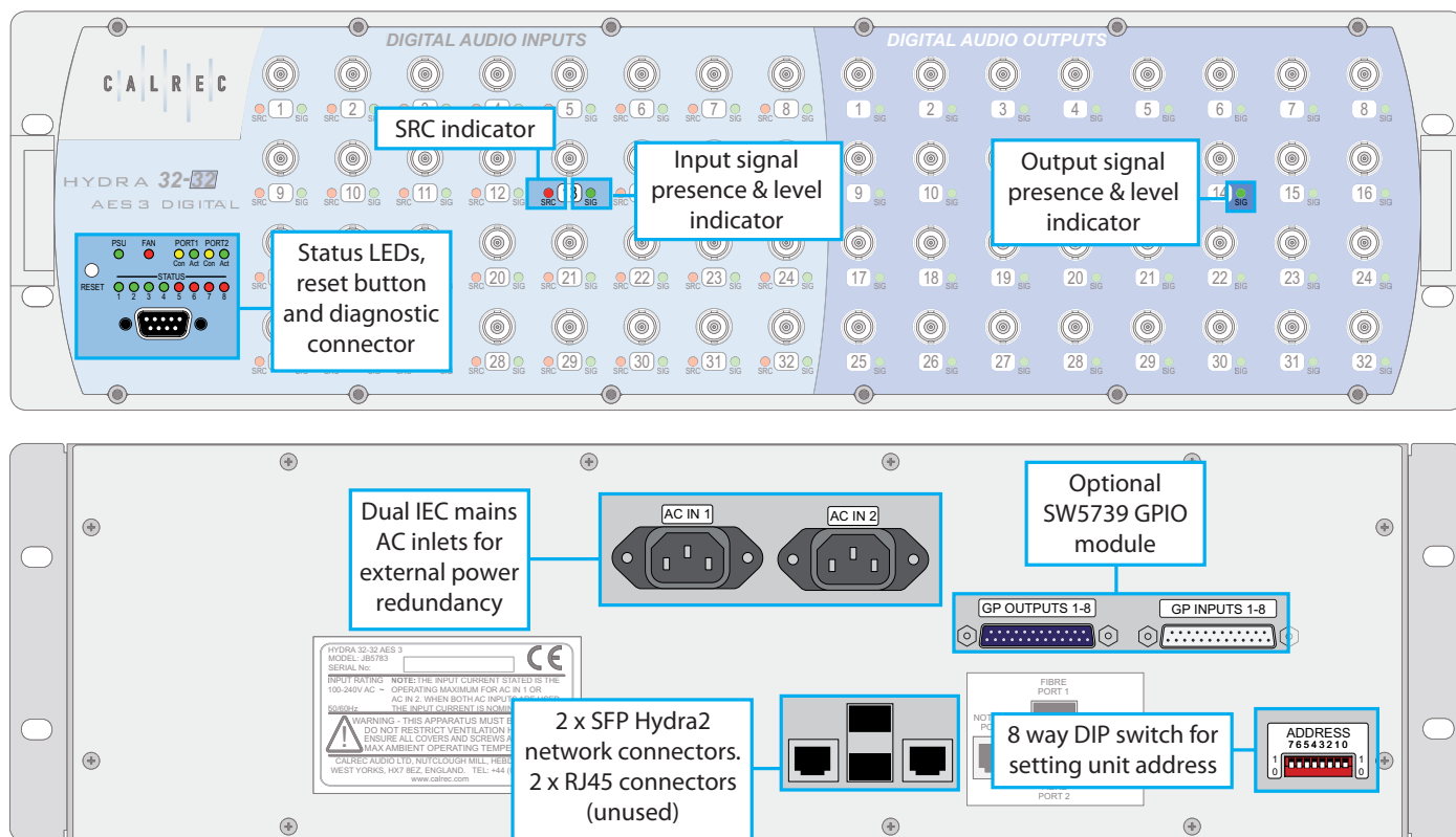
FIGURE 3 - JB5783 - 32 AES3 INPUTS, 32 AES3 OUTPUTS
