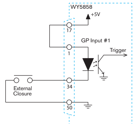
FIGURE 2 - INPUT WIRING EXAMPLE
