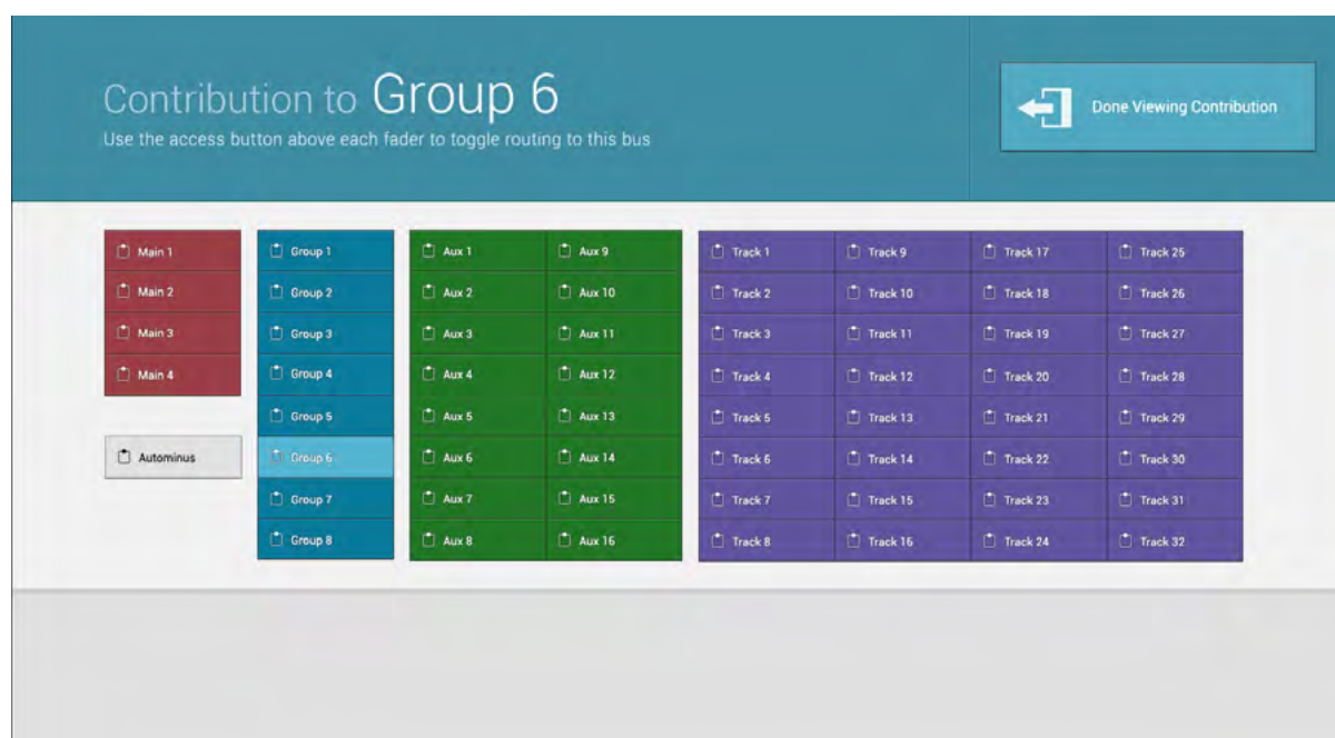
FIGURE 2 - CONTRIBUTION MODE—GROUP 6
