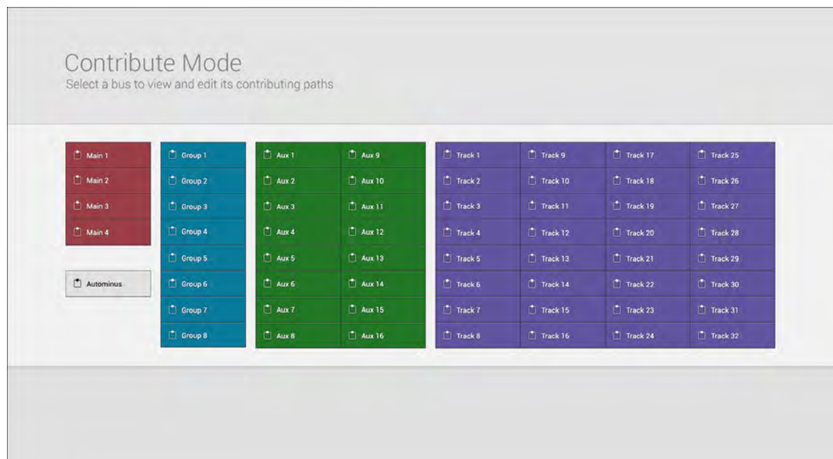
FIGURE 1 - CONTRIBUTION WINDOW
