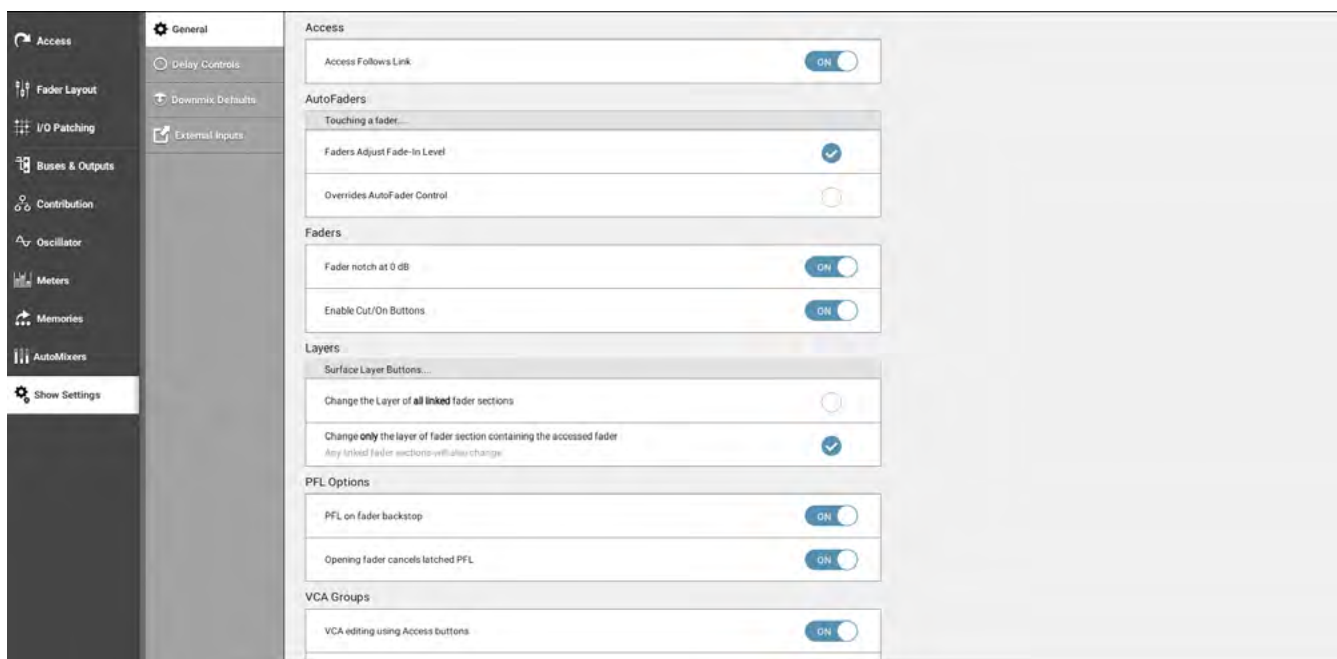
FIGURE 4 - SHOW SETTINGS
