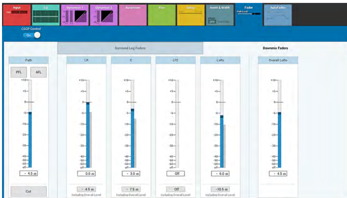
FIGURE 1 - DOWNMIX FADERS
