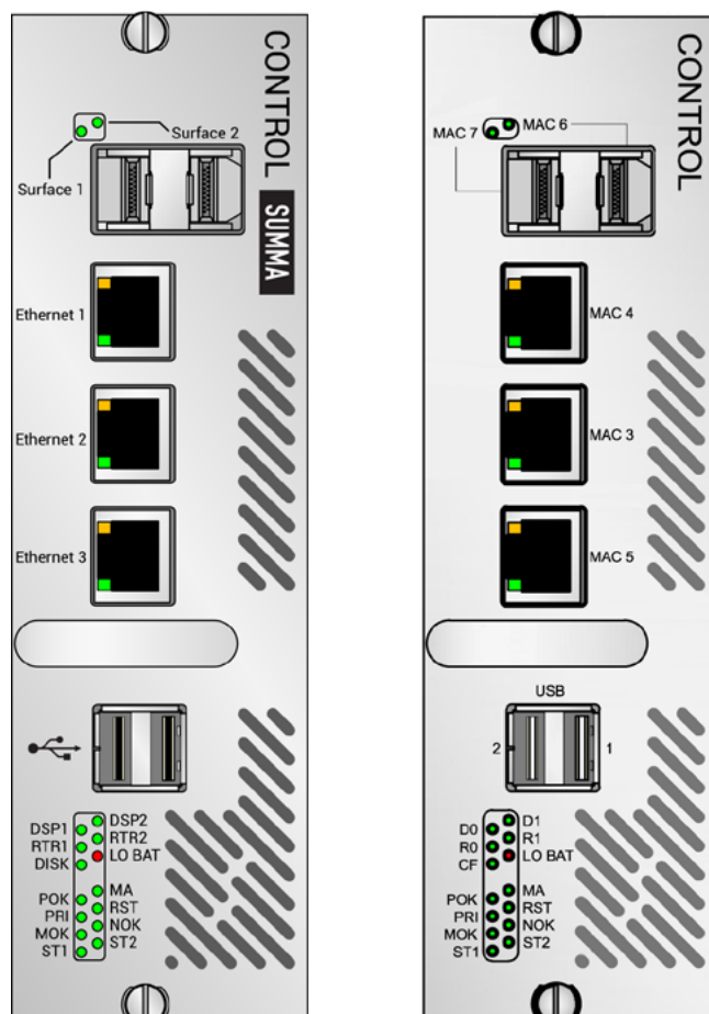
FIGURE 1 - CONTROL PROCESSORS
