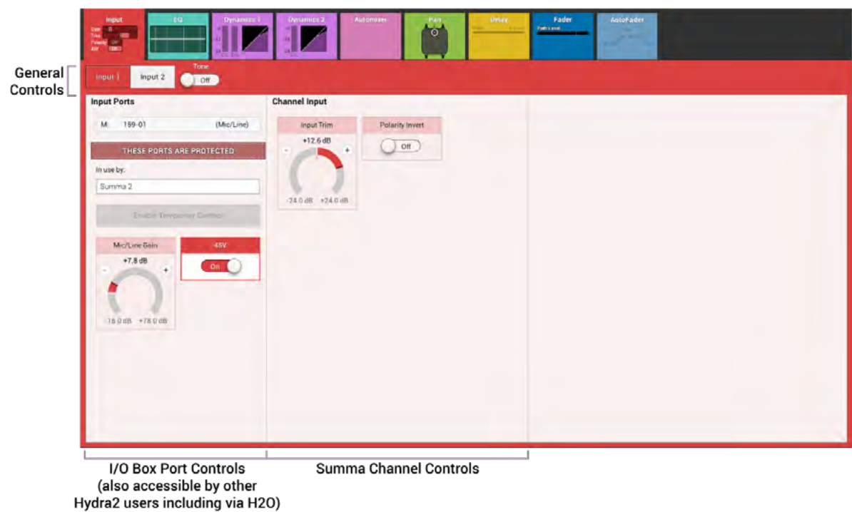
FIGURE 1 - INPUT CONTROLS
