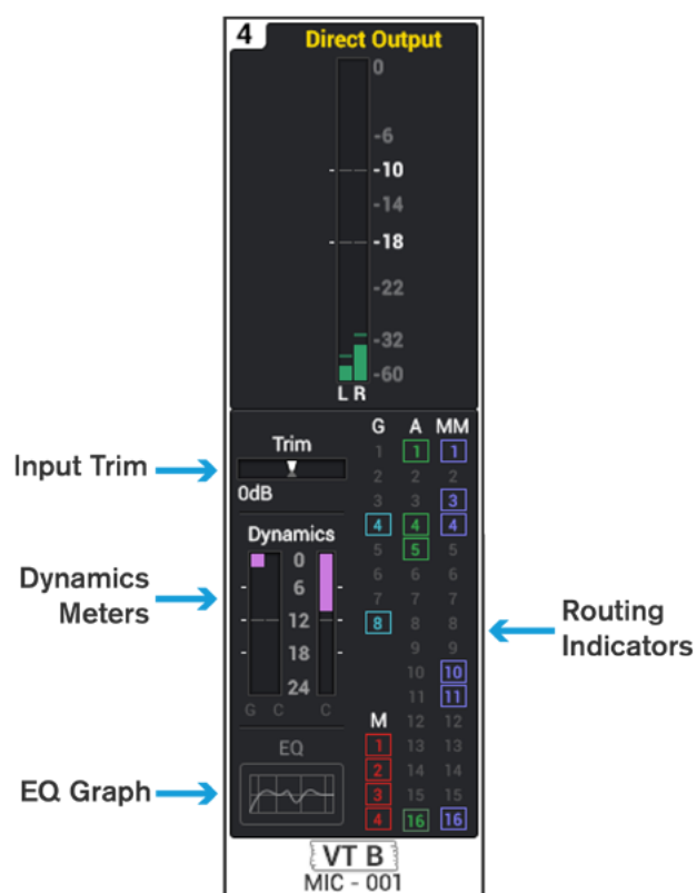
FIGURE 1 - FADER METER
