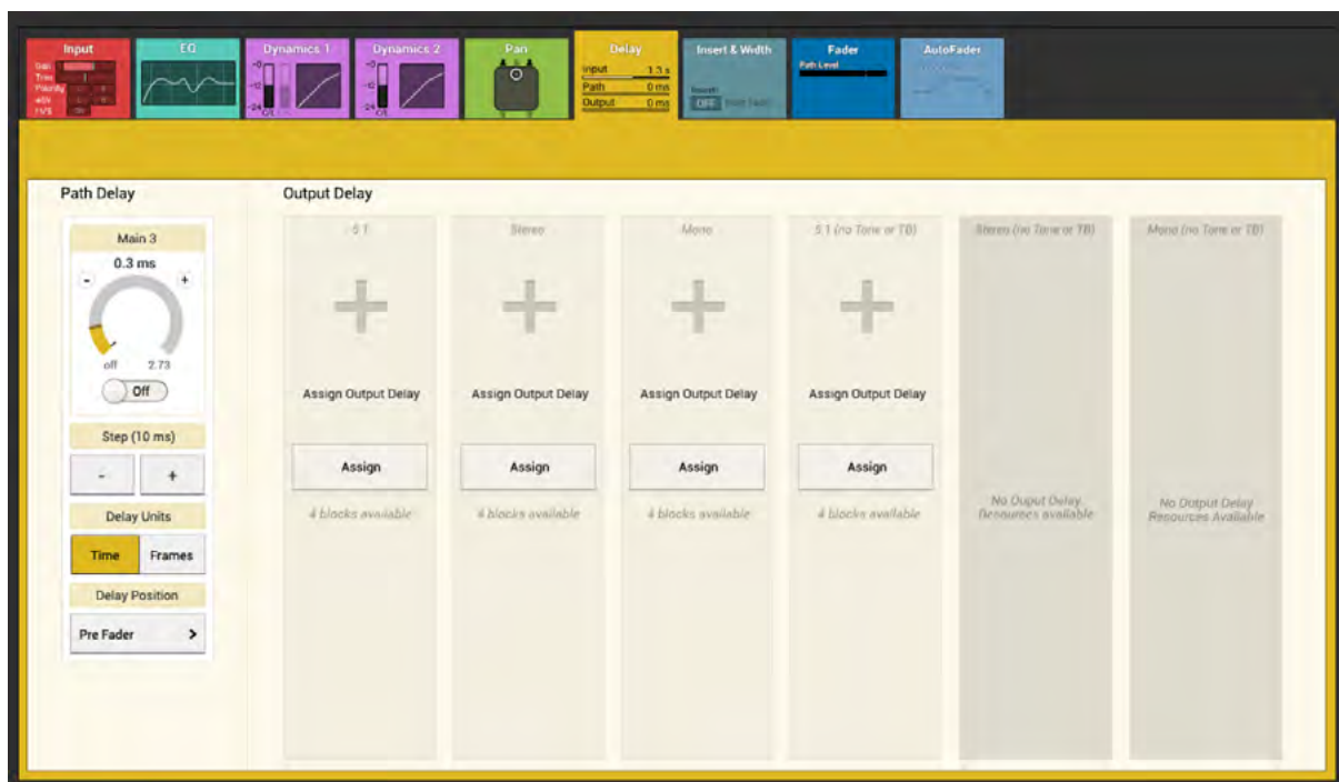
FIGURE 1 - DELAY CONTROLS
