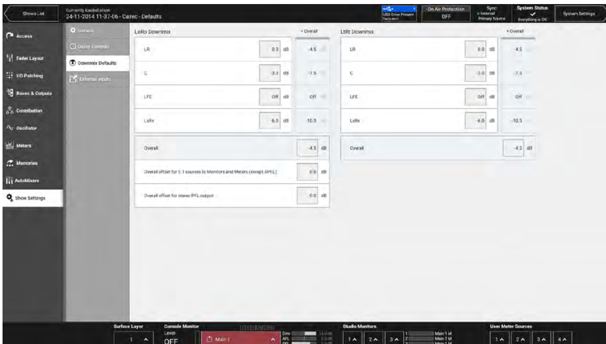
FIGURE 2 - DOWNMIX DEFAULTS
