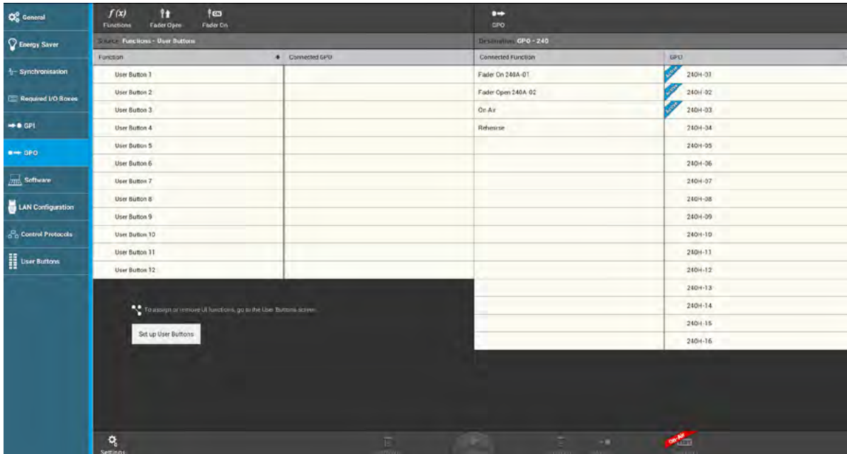
FIGURE 4 - GPO
