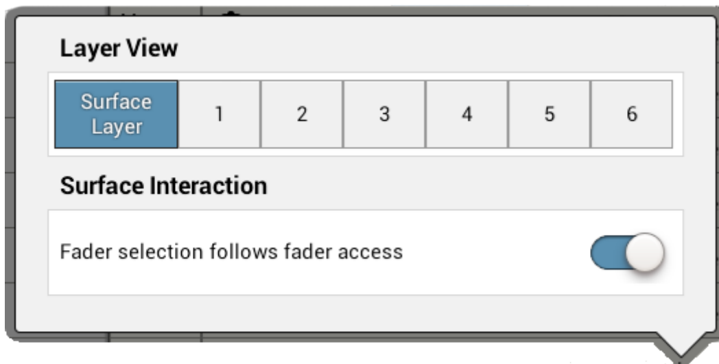
FIGURE 3 - SETTINGS POP-UP
