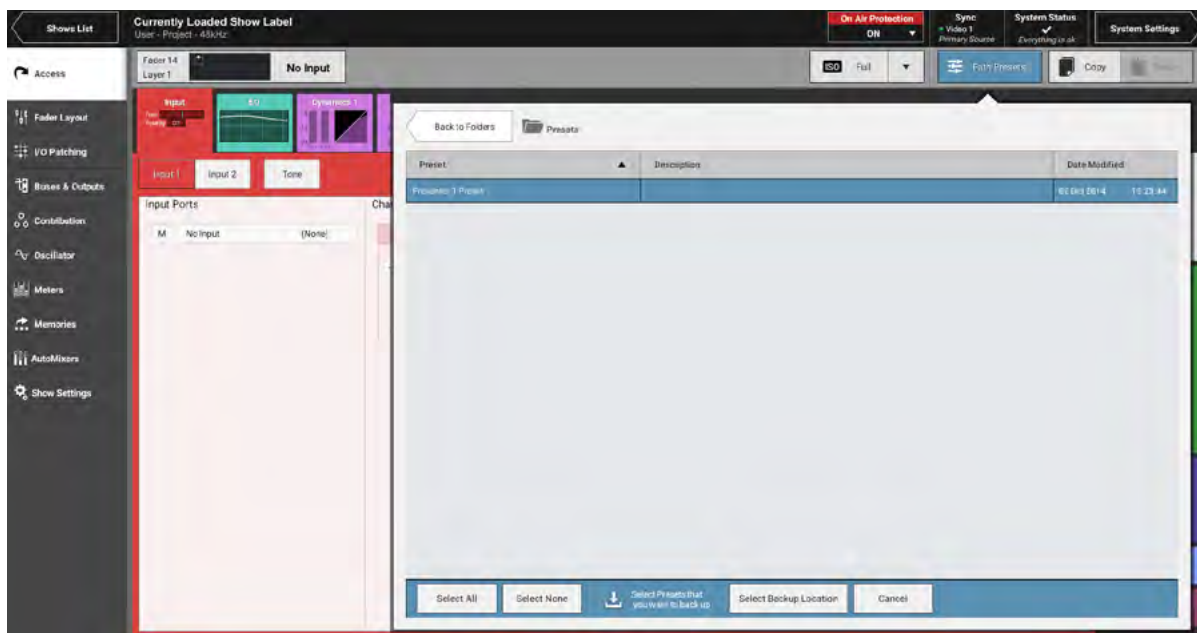
FIGURE 3 - BACKUP PRESETS
