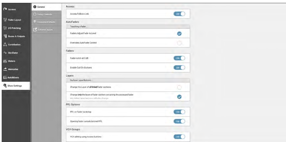
FIGURE 1 - LAYER SETTINGS
