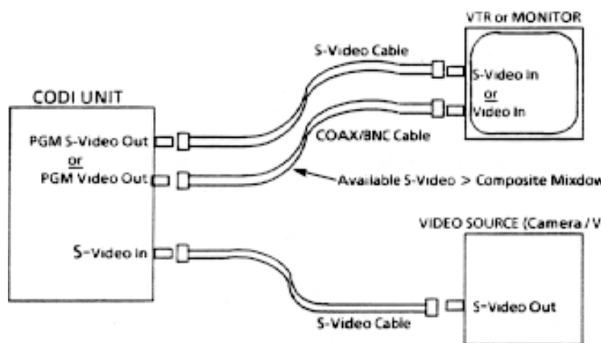
Figure 2-12. CODI Program Keyer Output Connection
