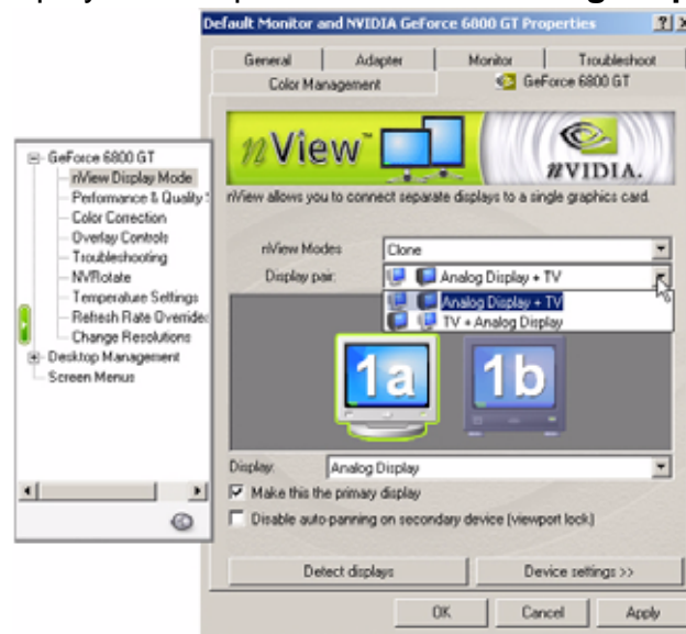
Figure 5-6. “nView Display Mode” controls on the GeForce 6800 GT tab
