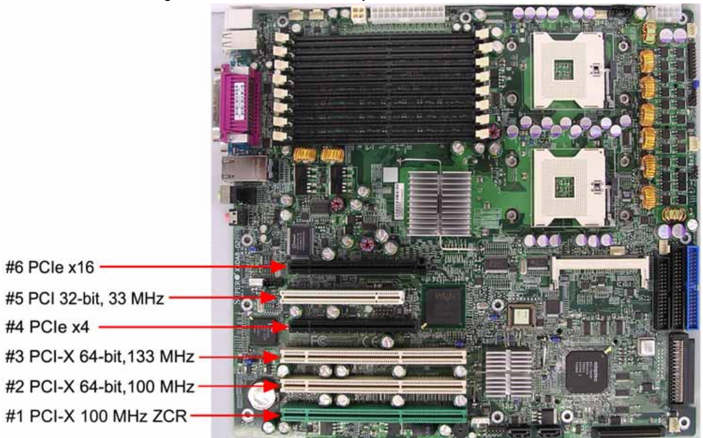
Figure 7-9. X6DA8-G2 expansion slots.
