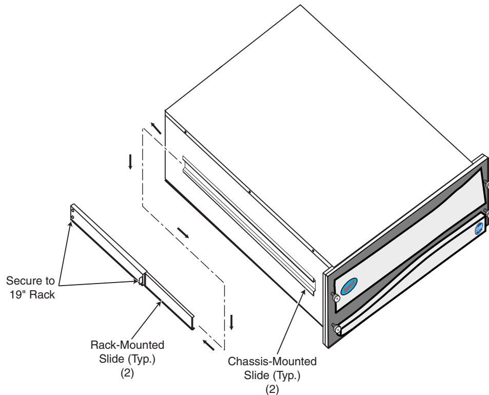
Figure 3-1. Duet HyperX and its rack-mounting hardware
