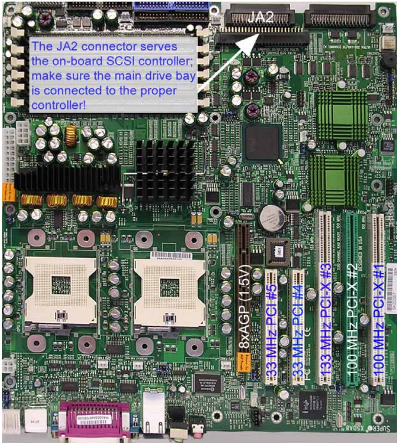
Figure 8-6. HyperX motherboard.
