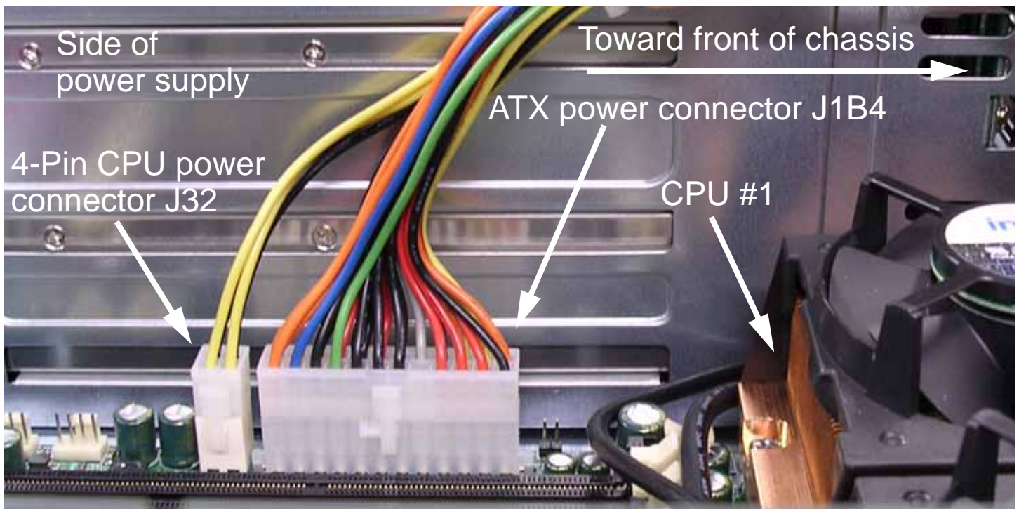
Figure 6-10. CPU power connector, left, with ATX power connector, center.
