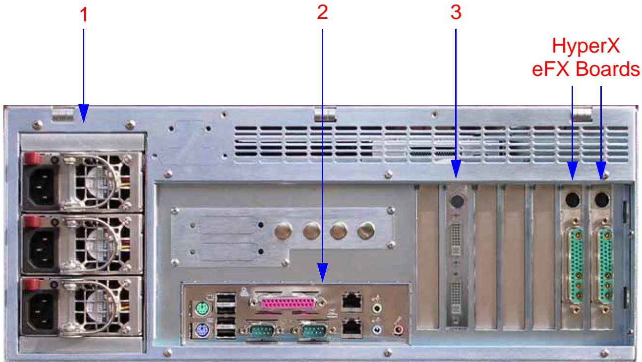
Figure 4-1. HyperX HD/SD with two eFX boards shown. Numbered components are common to all HyperX systems.
