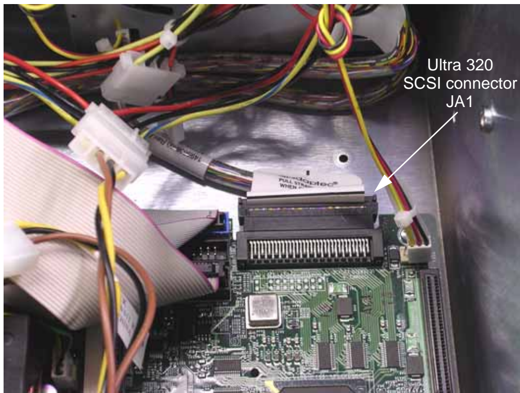
Figure 6-6. Close-up of SCSI connector JA1.
