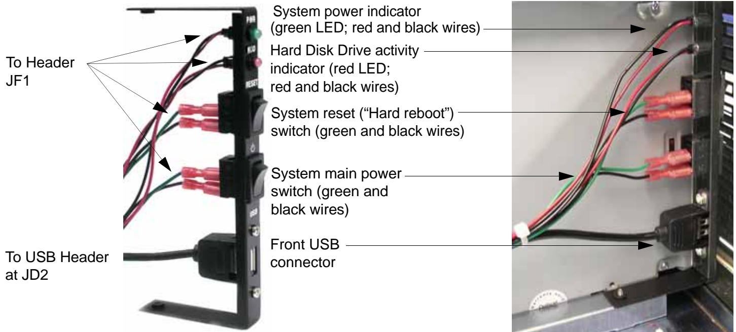
Figure 6-1. HyperX front panel, shown isolated at left and installed at right.
