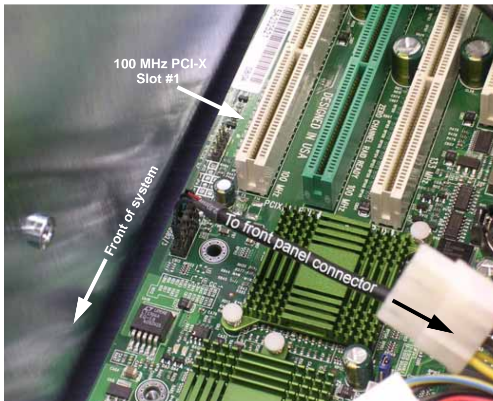
Figure 8-4. Close-up view of motherboard's USB connector
