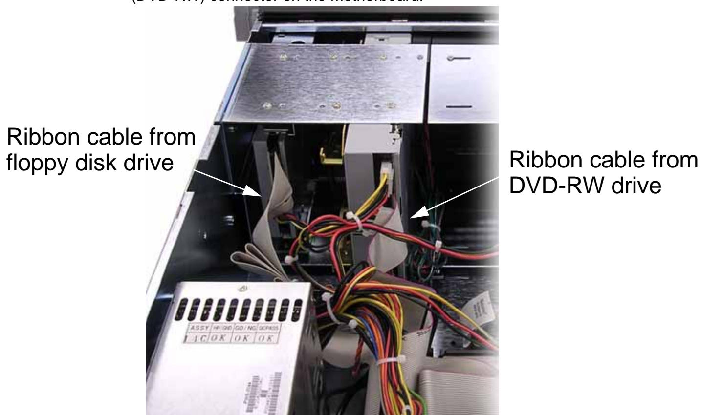
Figure 8-5. Rear view, floppy disk and DVD-RW drive cables
