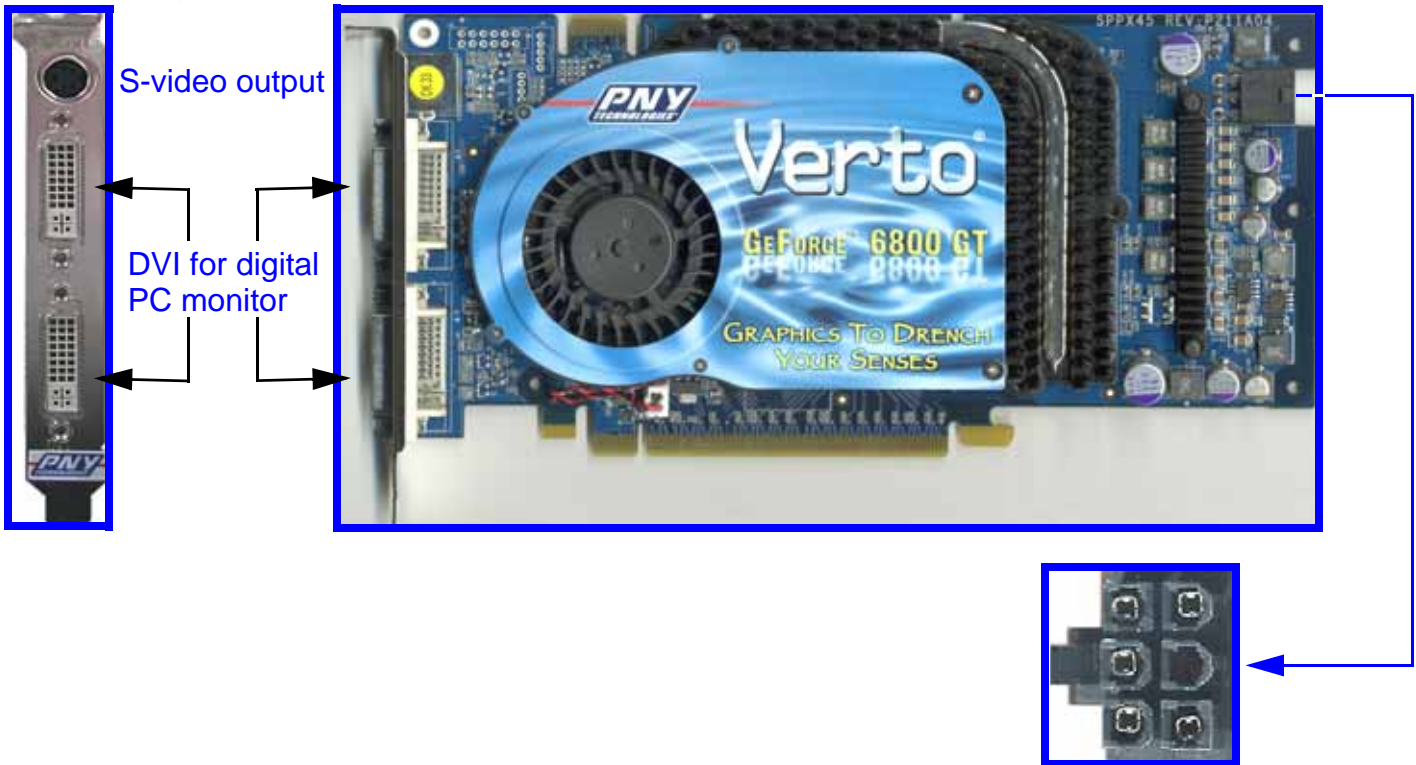
Figure 7-7. GeForce 6800 GT card. Left: Signal connectors. Bottom: Close-up of 5-pin Molex power connector.
