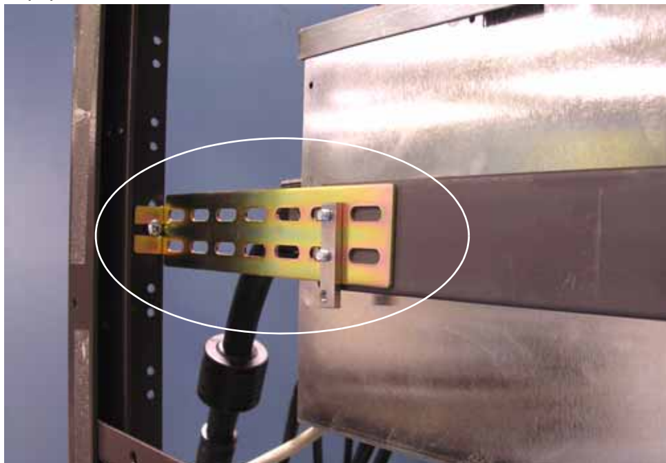
Figure 3-2. Extra brace added to rack slide.
