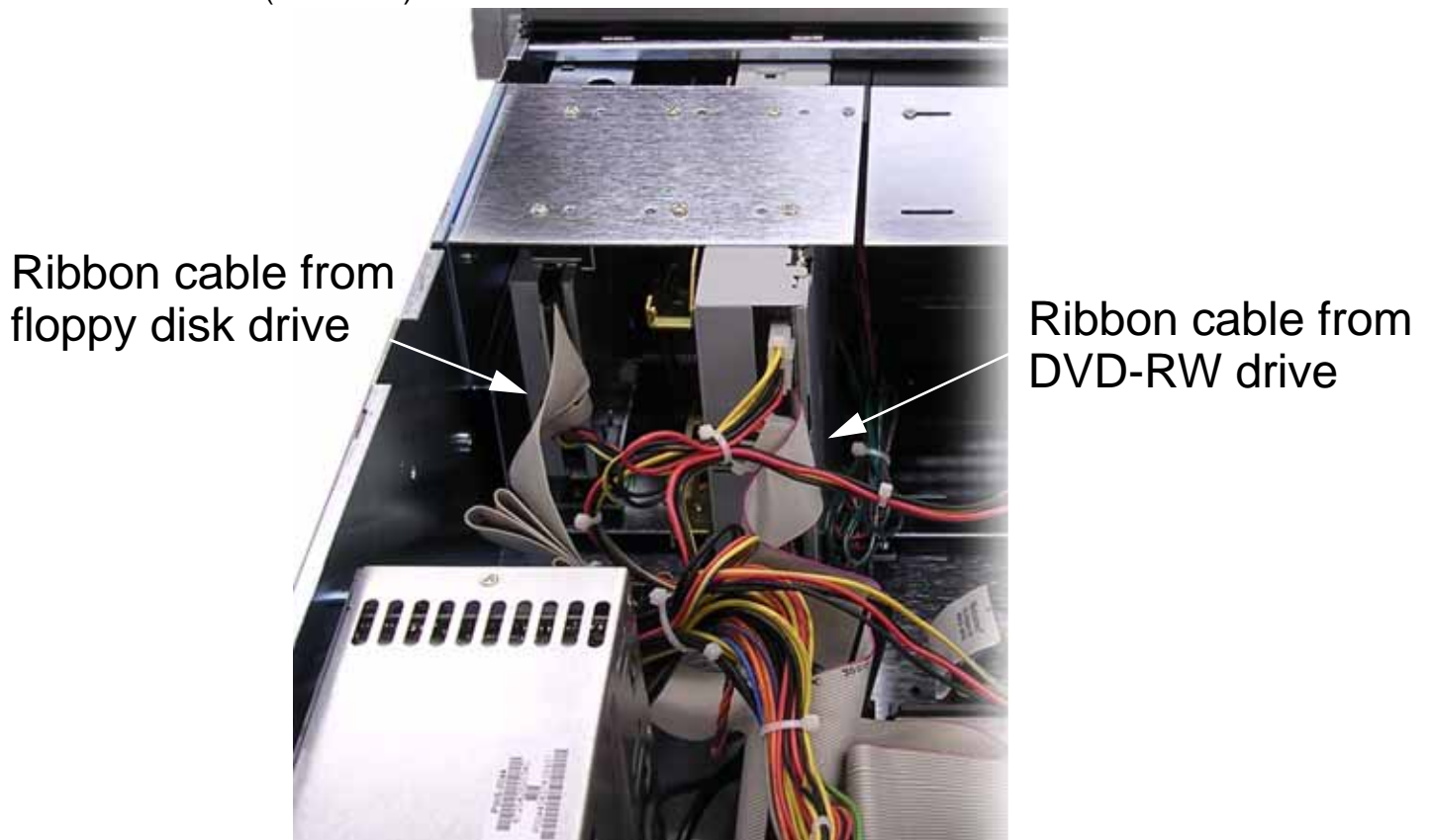
Figure 7-5. Rear view, floppy disk and DVD-RW drive cables
