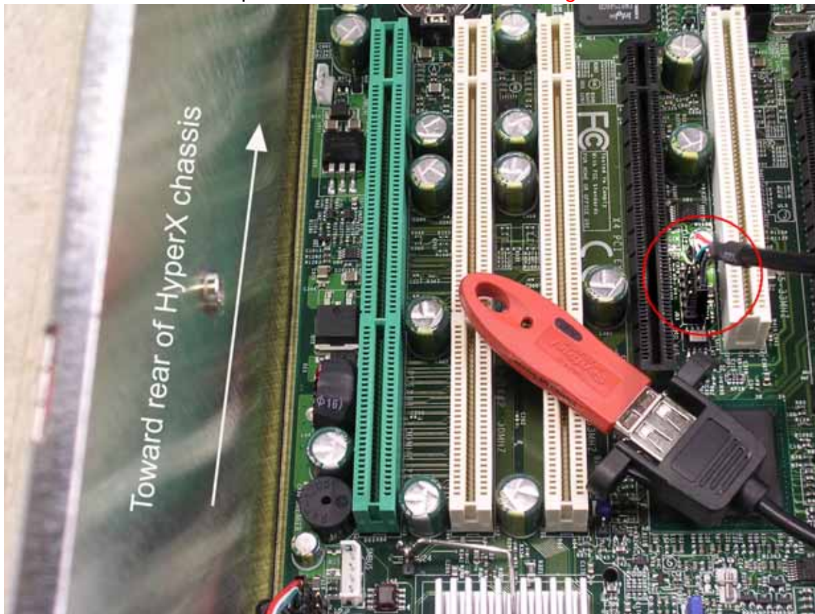
Figure 6-5. The FPUSB 4/5 header at JD3, located between slots #4 and #5. The red “dongle” security device, shown in foreground for reference, is located elsewhere in the system’s normal configuration.
