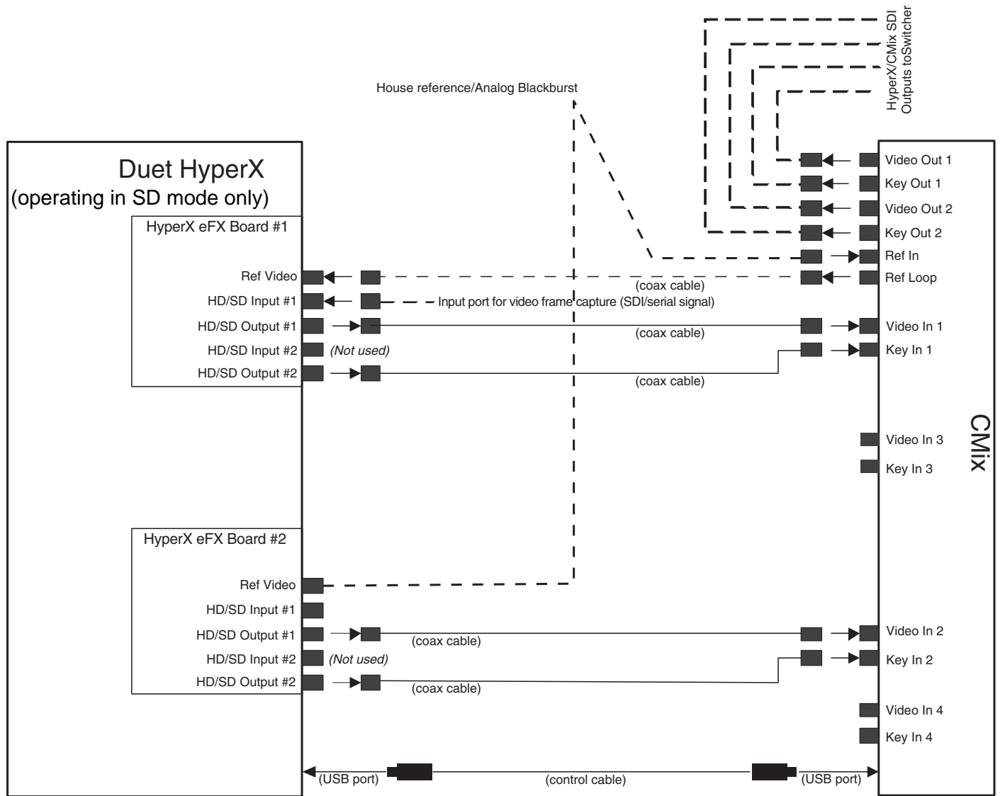
Figure 4-7. Typical connections between a two-channel standard-definition HyperX and Chyron's CMix
