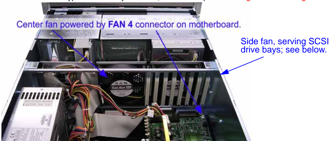
Figure 6-12. Power connection to center system fan
