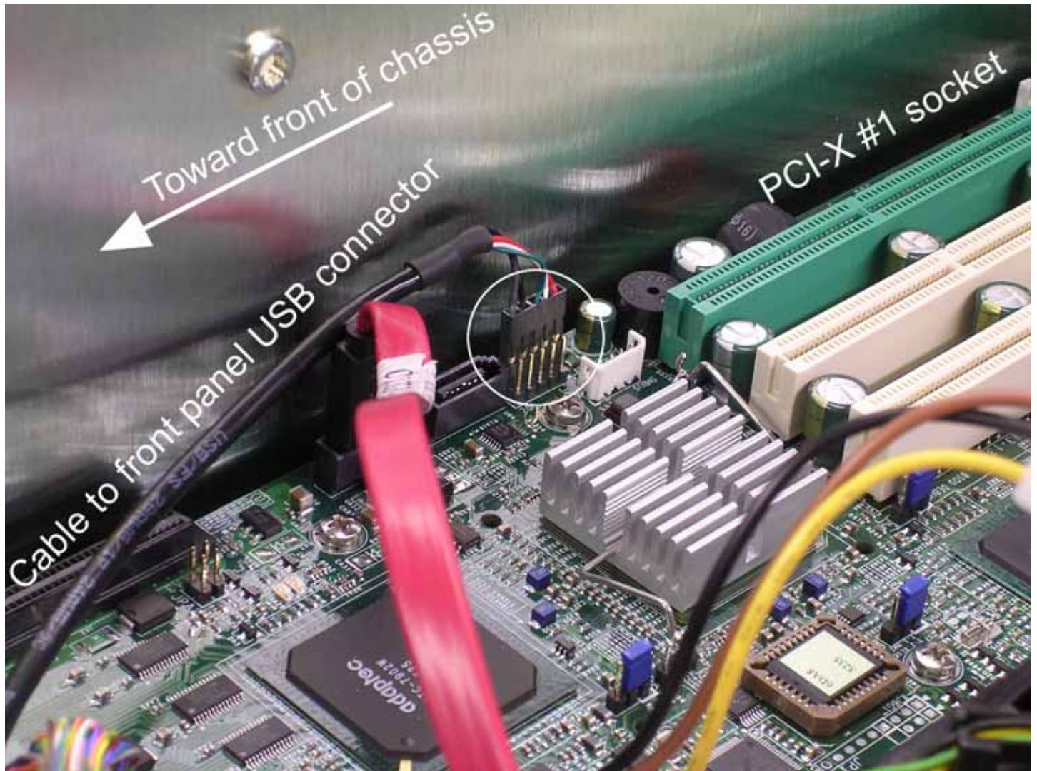
Figure 7-4. Close-up view of motherboard's USB connector, circled. Note that the black cable goes to the front USB connector.
