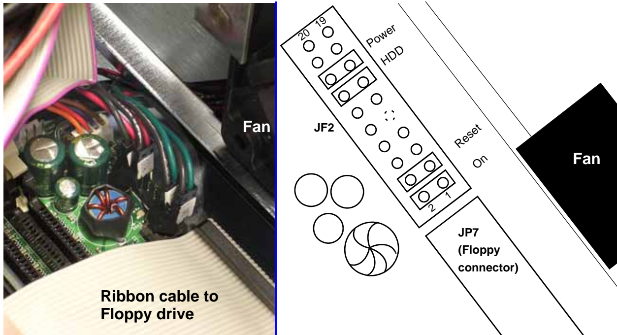
Figure 8-3. Header JF2, close-up, at left. Labelled sketch at right.
