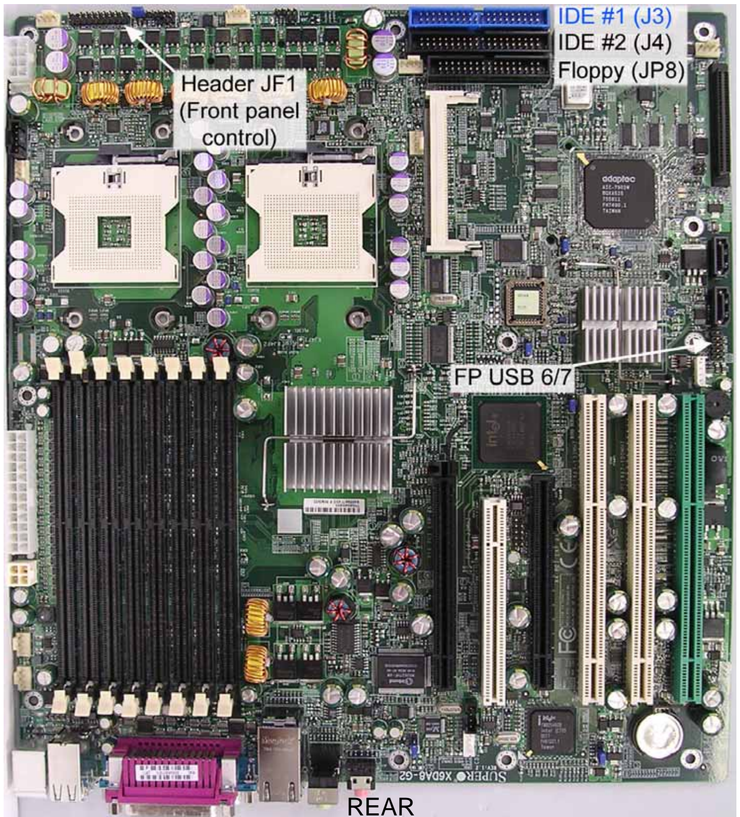
Figure 7-2. X6DA8-G2 motherboard
