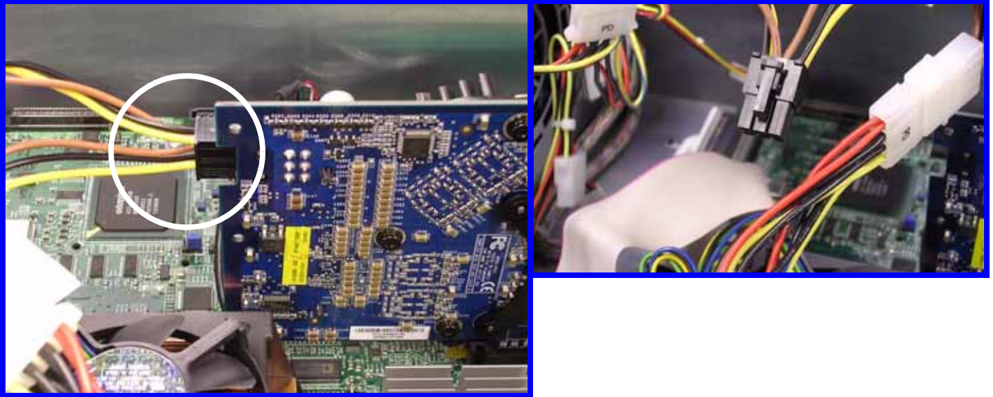
Figure 7-8. The graphics card's Molex power connector. At right, the connector is seen close-up, disconnected to show details.
