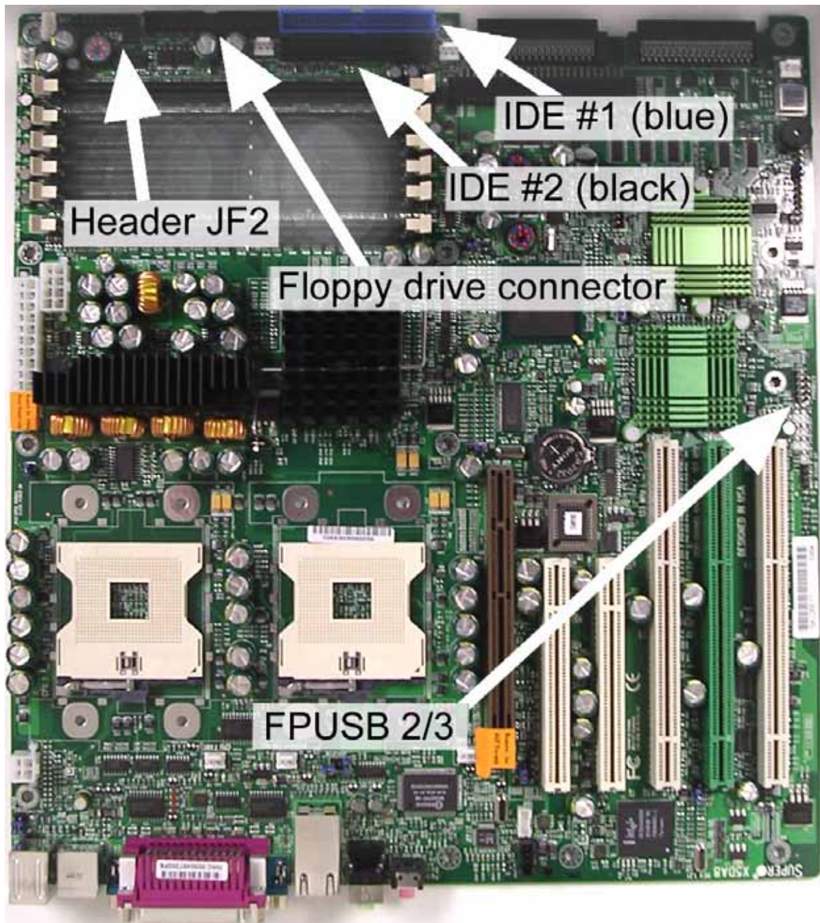
Figure 8-2. X5DA8 motherboard
