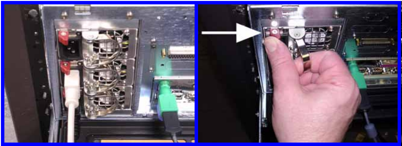
Figure 6-8. Replacing a power supply module
