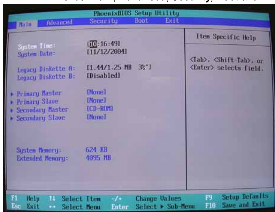
Figure 6-14. BIOS main screen
