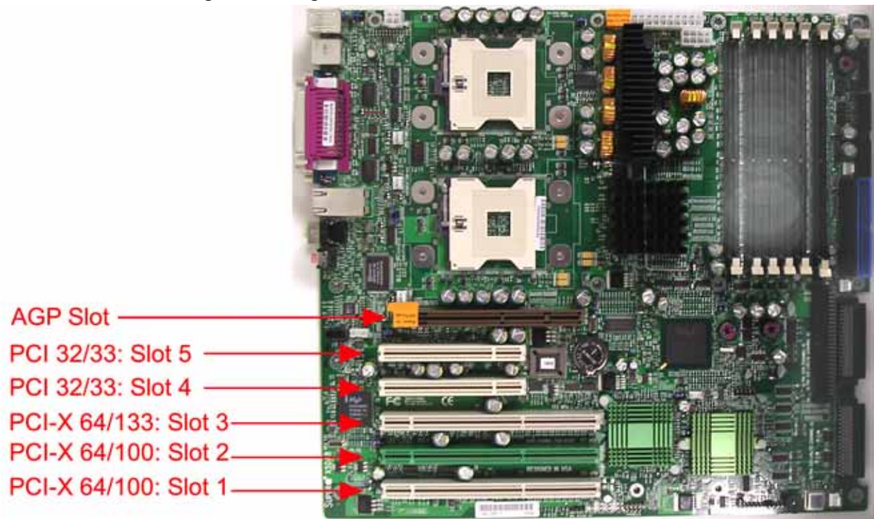
Figure 8-8. PCI and PCI-X slots, numbered at right
