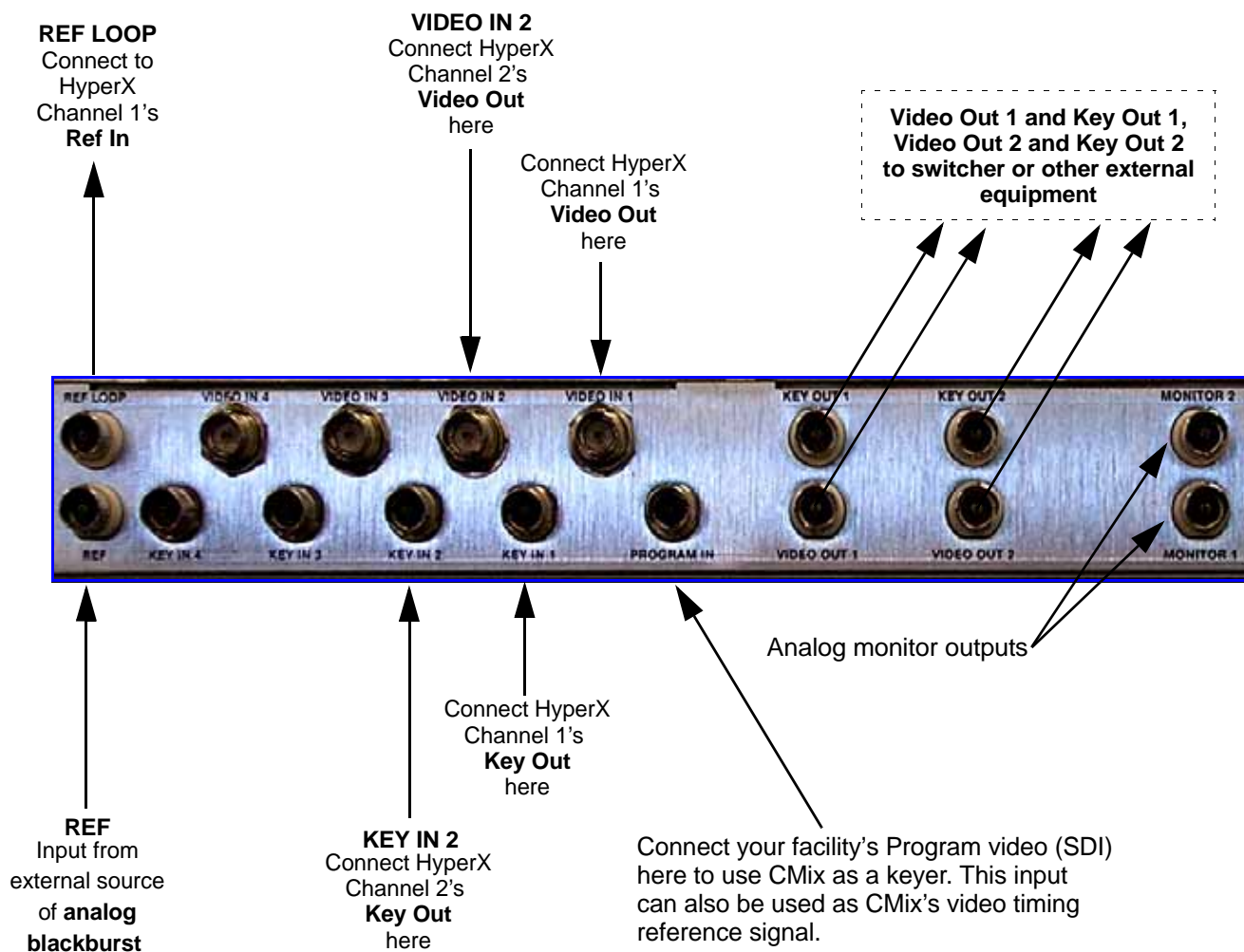
Figure 4-6. Chyron CMix rear panel with typical connections to a two-channel standard-definition HyperX system
