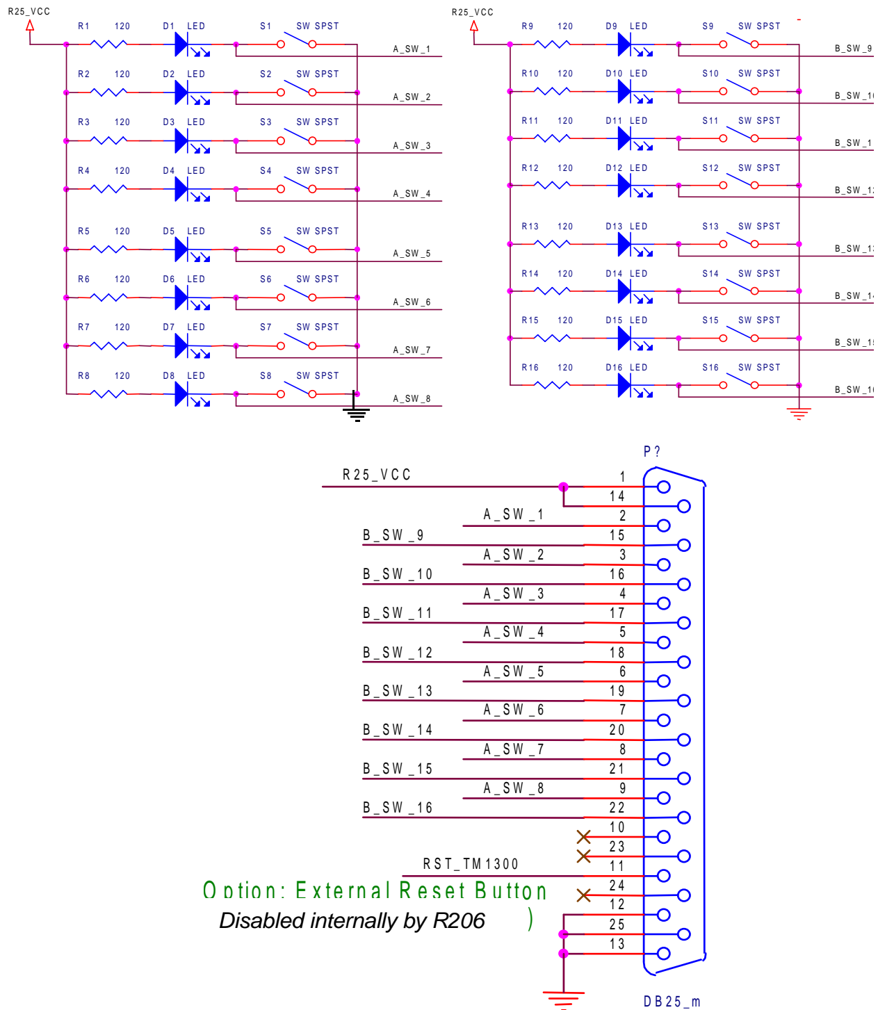
Figure 9-1. 16-Port GPIO Adapter Cabling
