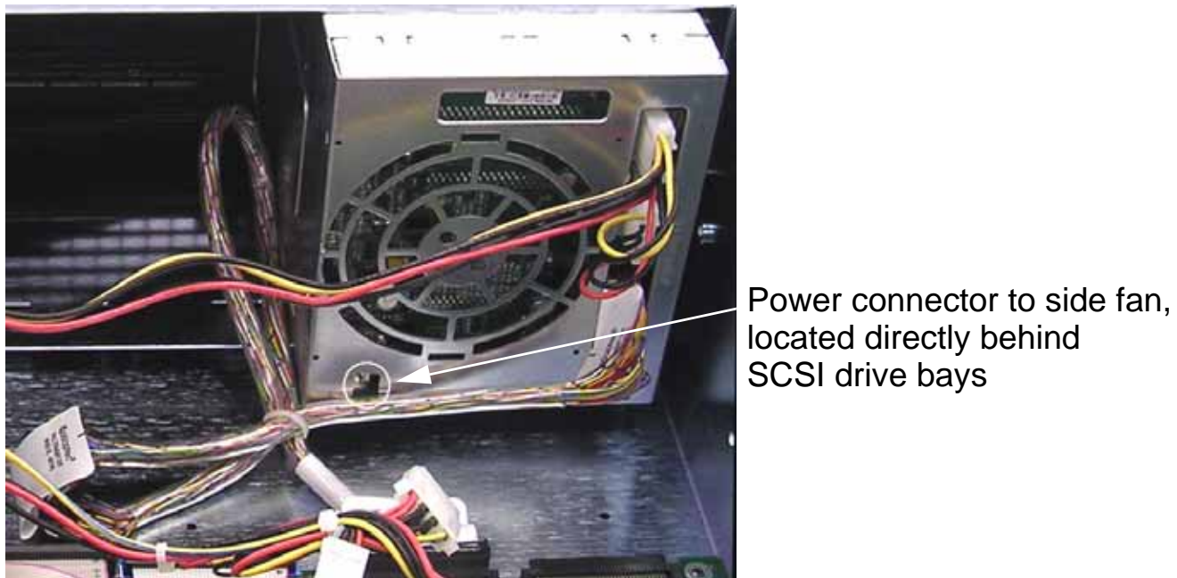
Figure 6-13. Power connection to “outer fan” which serves SCSI drive bays
