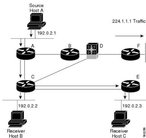
Figure 2: Source Tree
