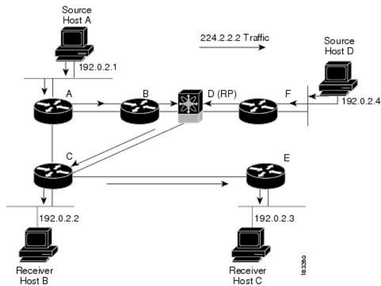
Figure 3: Shared Tree
