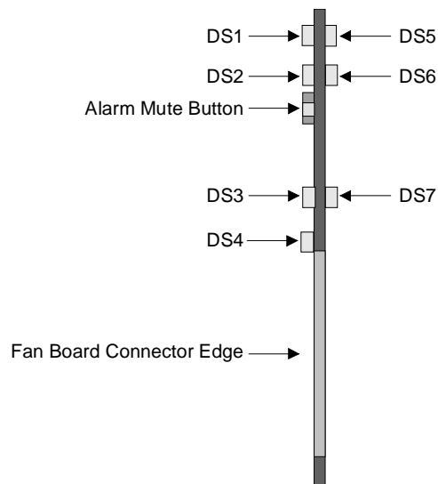
Figure 14. MFC-8310-N Card Edge Controls
