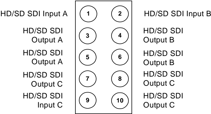
Figure 3. BNC Designations for the Card Rear Module RM-9005-A or 8310-RM-100
