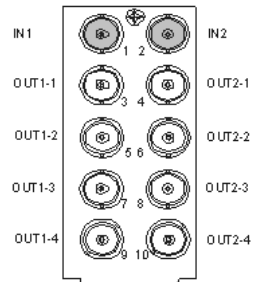
Figure 2. RM-9253-A Rear Module
