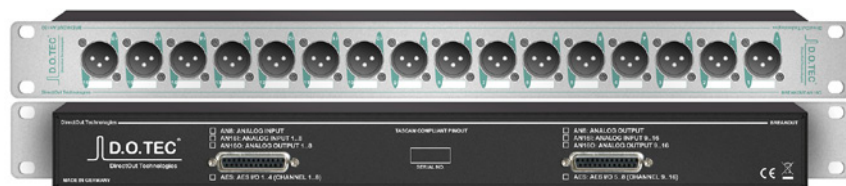
BREAKOUT.AN16O - analog output, 16 channels
