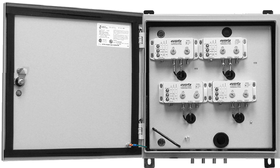
Figure 1-2: 2400ODU, Front Door Open, Swing Panel with 2408LT's Mounted
