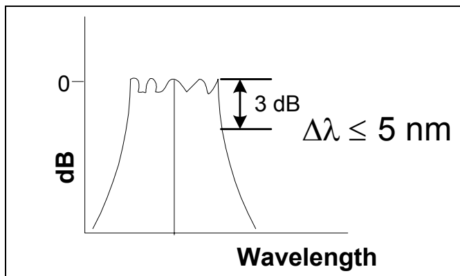
Figure A-4: Spectrum of FP Laser used in EO3F and EO3F-HD
