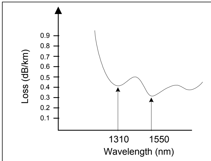
Figure A-2: Cables Losses at Various Wavelengths
