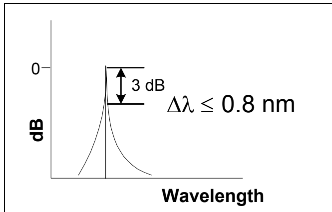
Figure A-3: Spectrum of DFB Laser used in EO3D-HD, EO5D-HD and EOxx-HD
