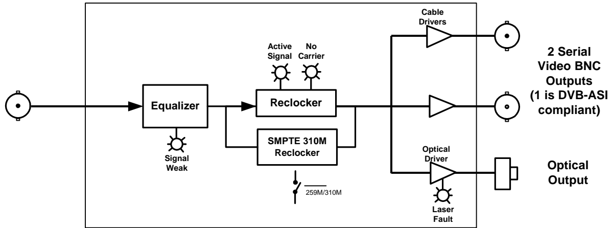
Figure 1-1: 2405EO Block Diagram
