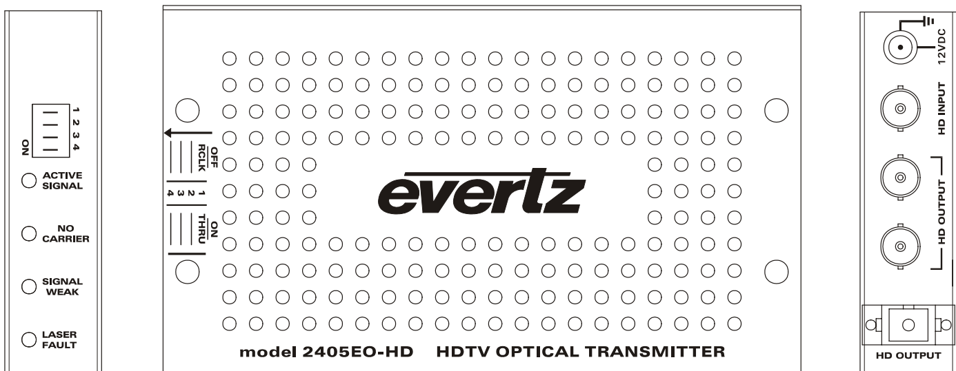
Figure 2: 2405EO-HD Module
