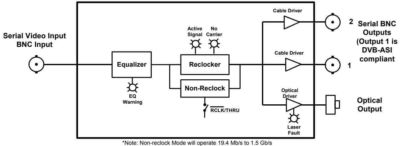
Figure 1: 2405EO-HD Block Diagram
