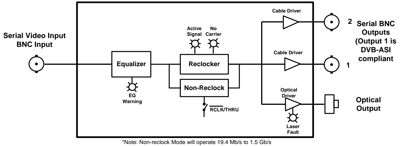
Figure 1-1: 2405EO-HD Block Diagram
