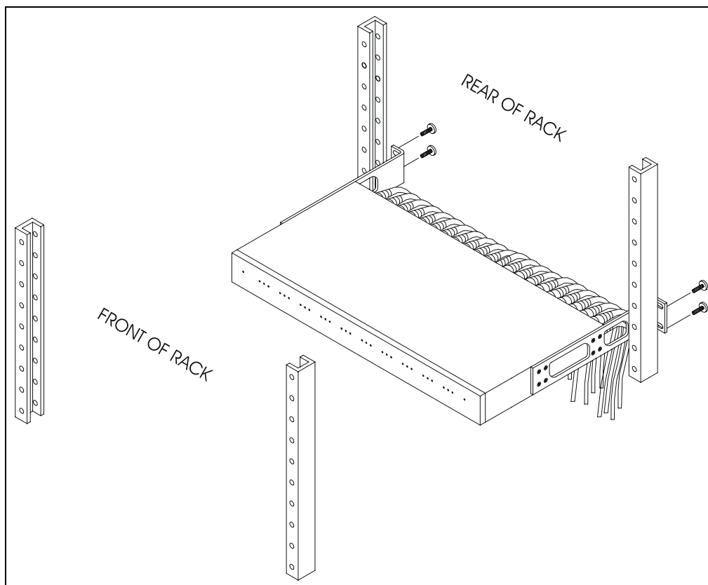
Figure 2-4: Rear Mounting
