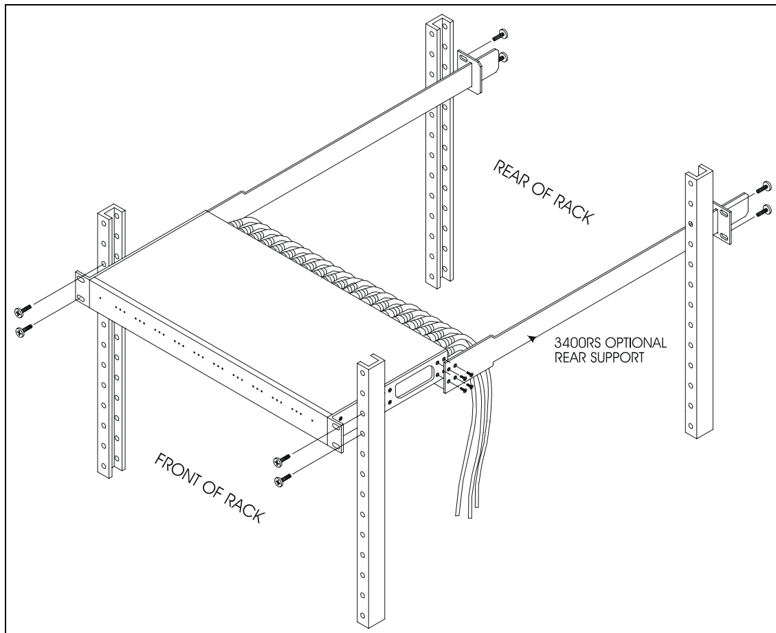
Figure 2-3: Front Mounting
