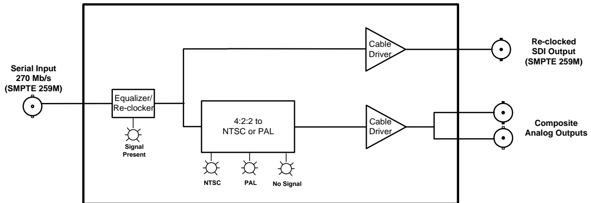
Figure 1-1: Block Diagram
