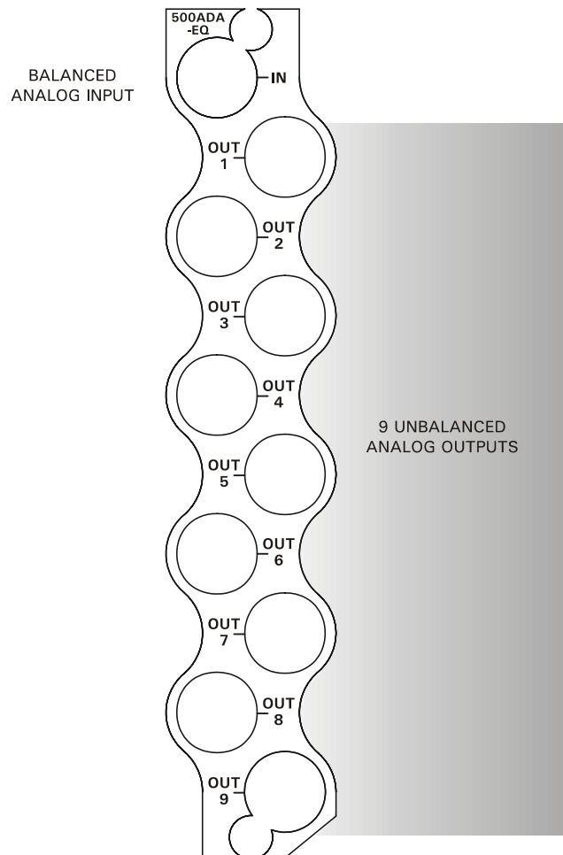
Figure 2: 500ADA-EQ Rear Panel Overlay
