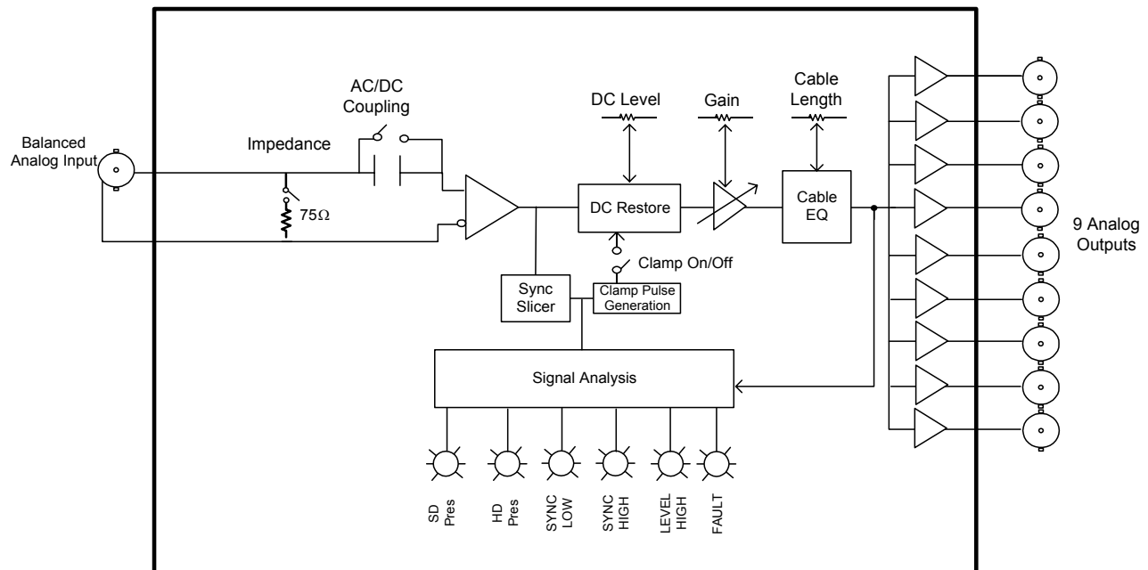
Figure 1: 500ADA-EQ Block Diagram
