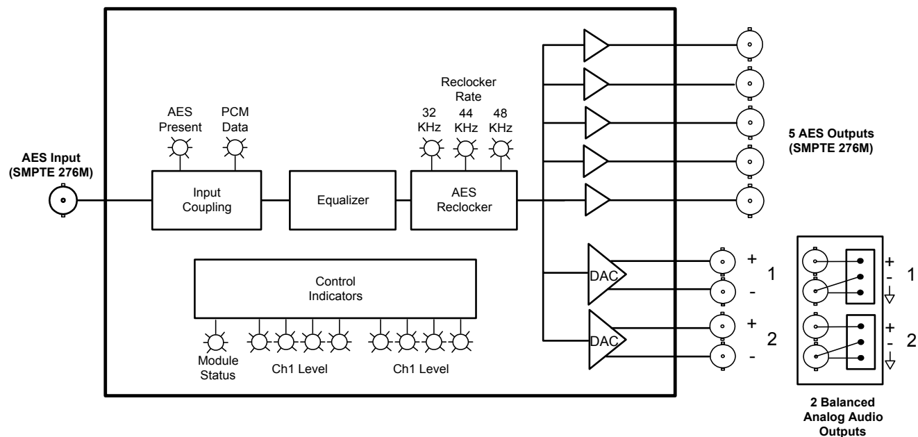
Figure 1: 500AMDA-AESU Block Diagram
