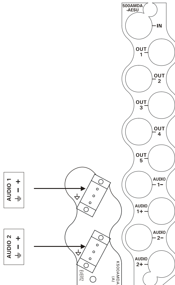
Figure 2: 500AMDA-AESU Rear Panel Overlay
