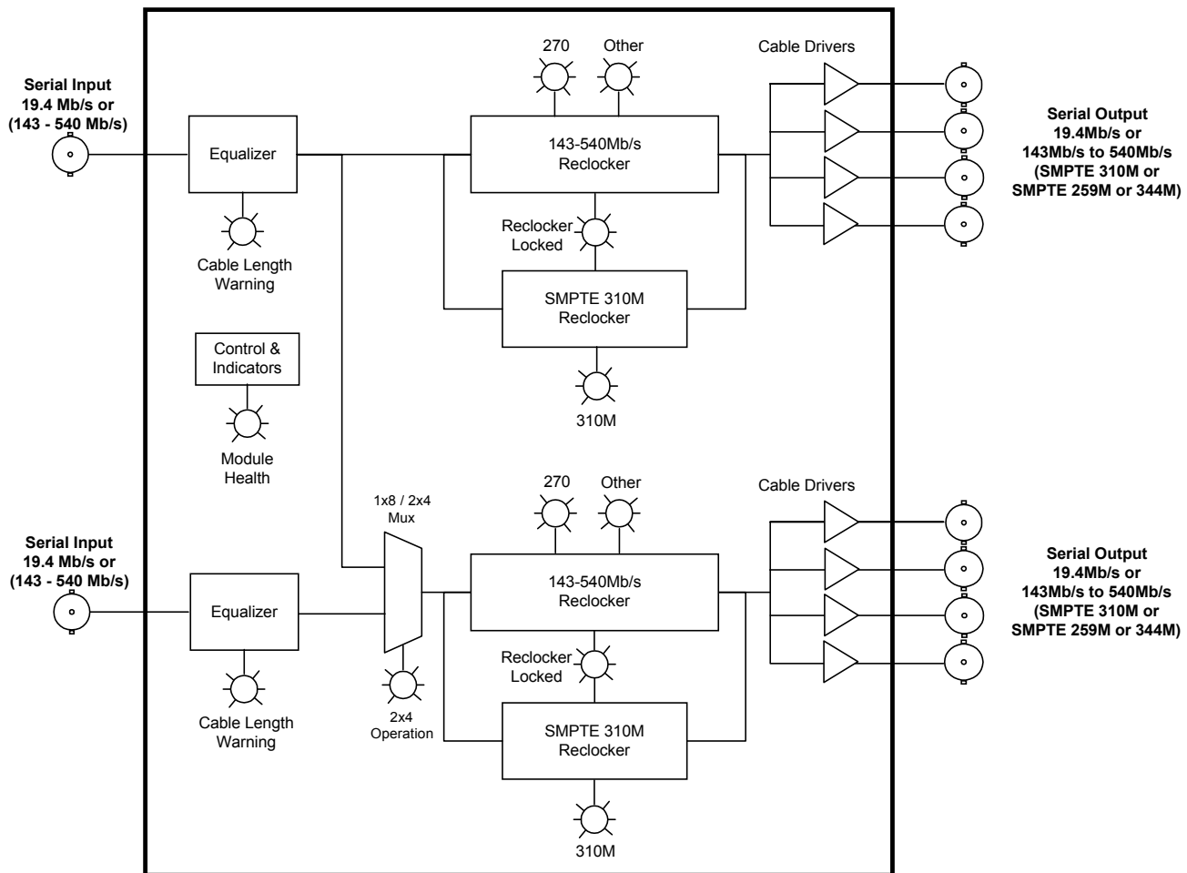
Figure 1: 500DA2Q Block Diagram
