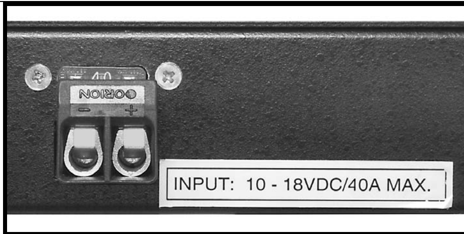
Figure 2: DC Input Connector and Fuse
