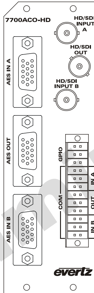
Figure 2: Rear Panel
