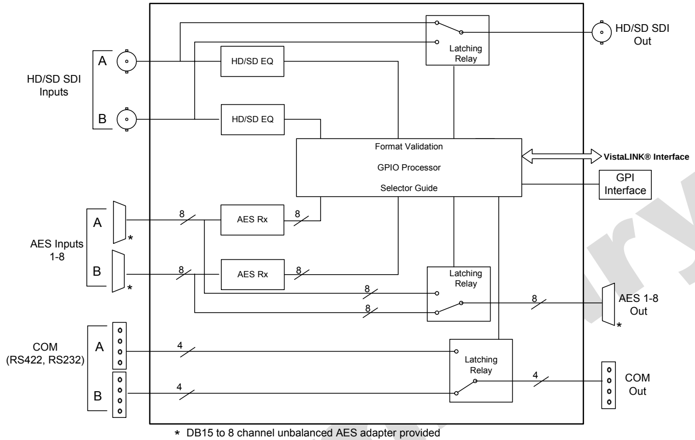
Figure 1: 7700ACO-HD Block Diagram
