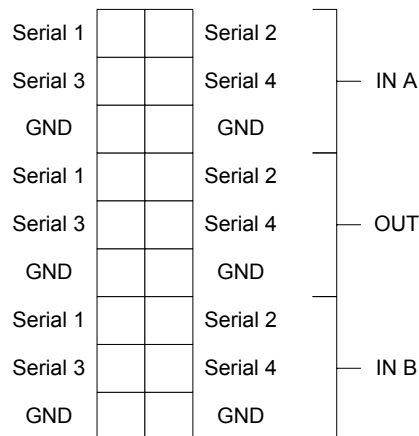
Figure 3: Control Connection Pin Out
