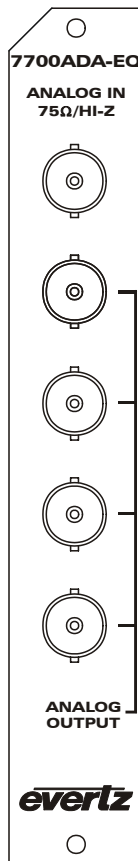
Figure 2: 7700ADA-EQ Rear Panel
