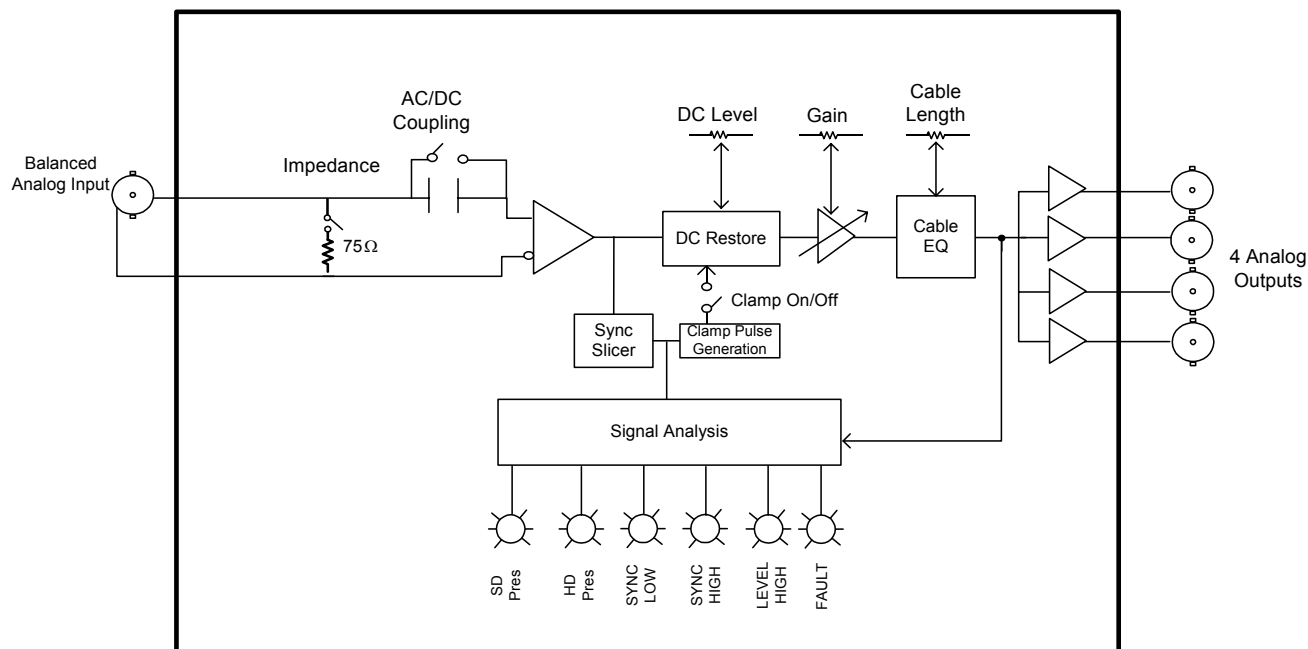
Figure 1: 7700ADA-EQ Block Diagram
