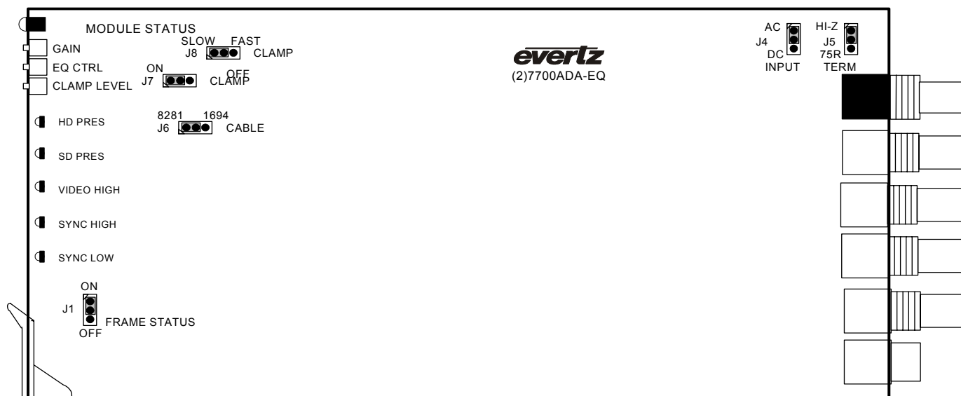
Figure 3: LED and Jumper Locations
