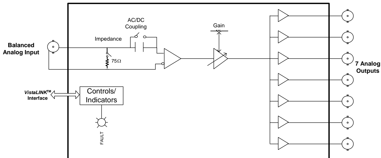
Figure 1: 7700ADA7 Block Diagram
