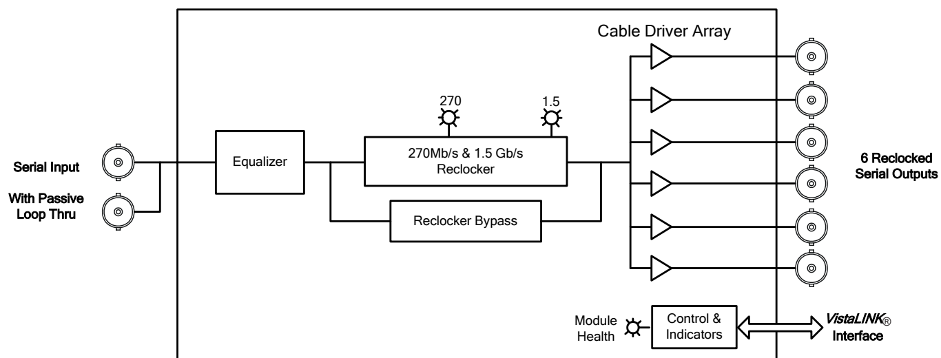
Figure 1-1: 7700DA6-HD-L Block Diagram
