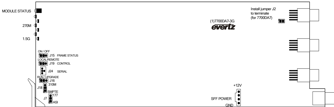
Figure 5-1: LED and Jumper Locations
