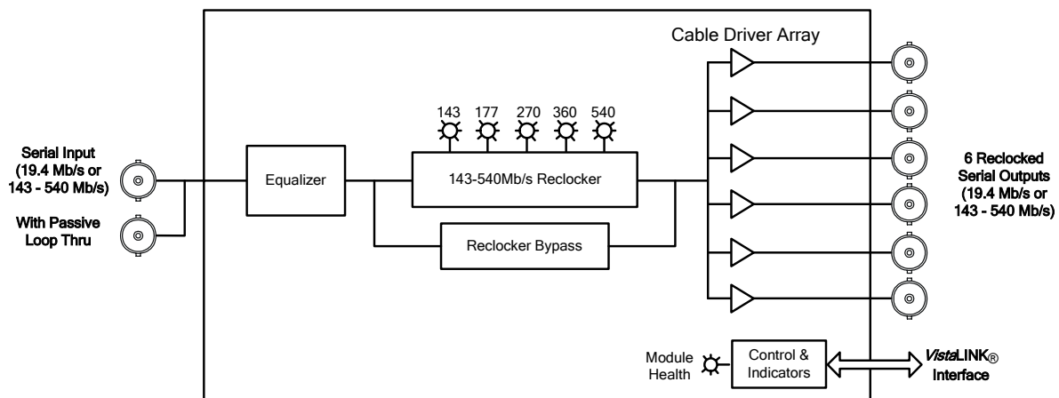
Figure 1-1: 7700DA6-L Block Diagram
