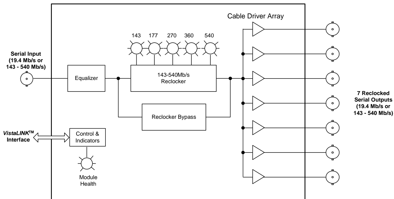
Figure 1: 7700DA7 Block Diagram
