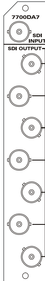
Figure 2: 7700DA7 Rear IO Module
