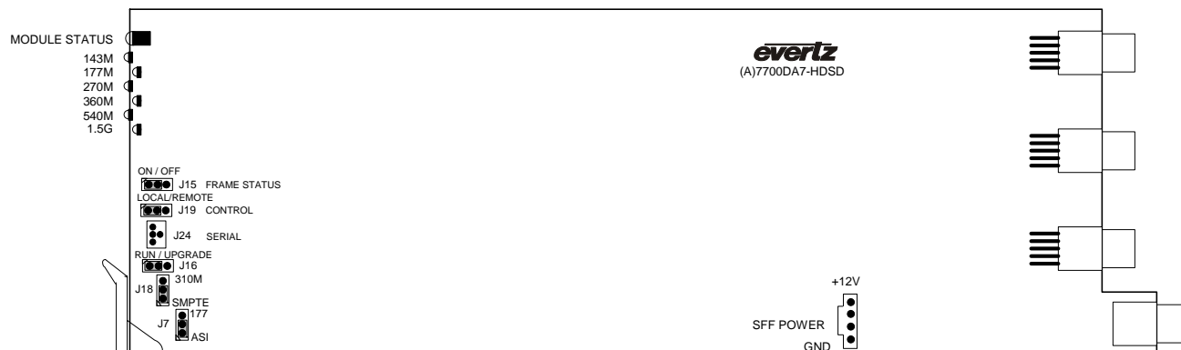
Figure 5-1: LED and Jumper Locations
