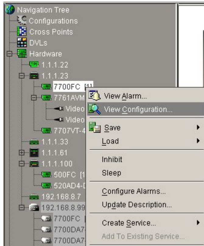
FC shown in the hardware tree
