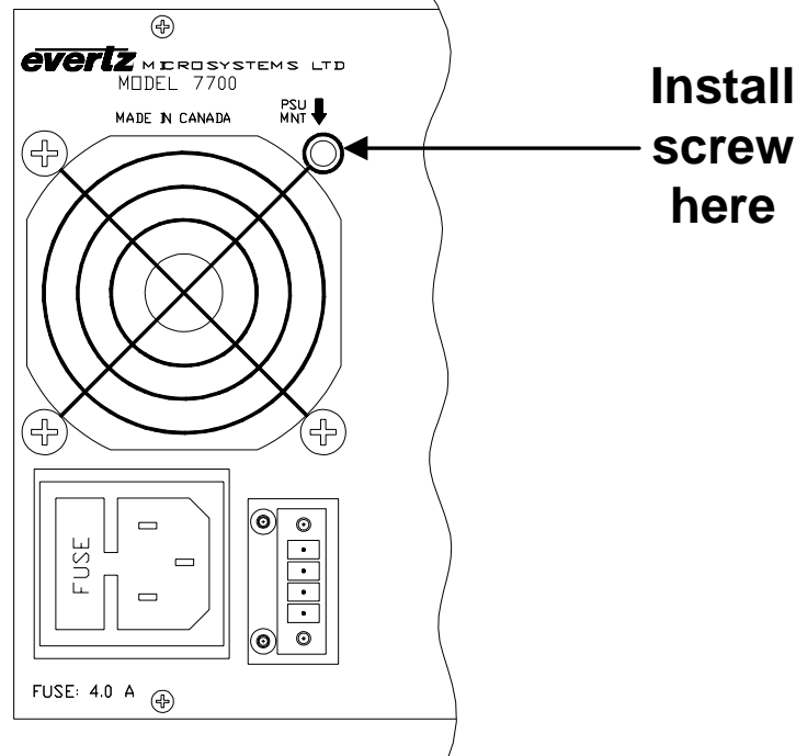
Figure 4: Locating the Power Supply Mounting Screw
