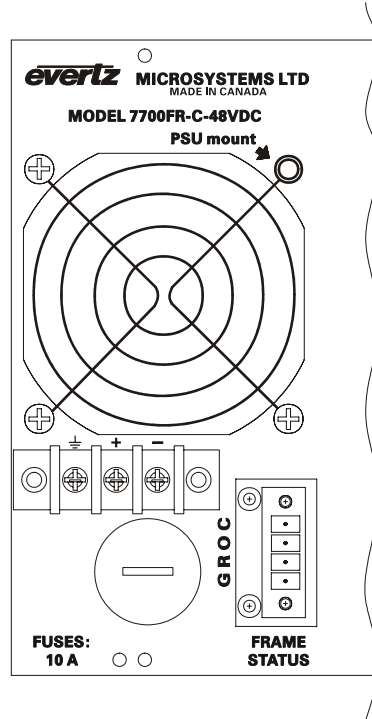
Figure 1-2: 7700FR-C-48VDC Rear Panel
