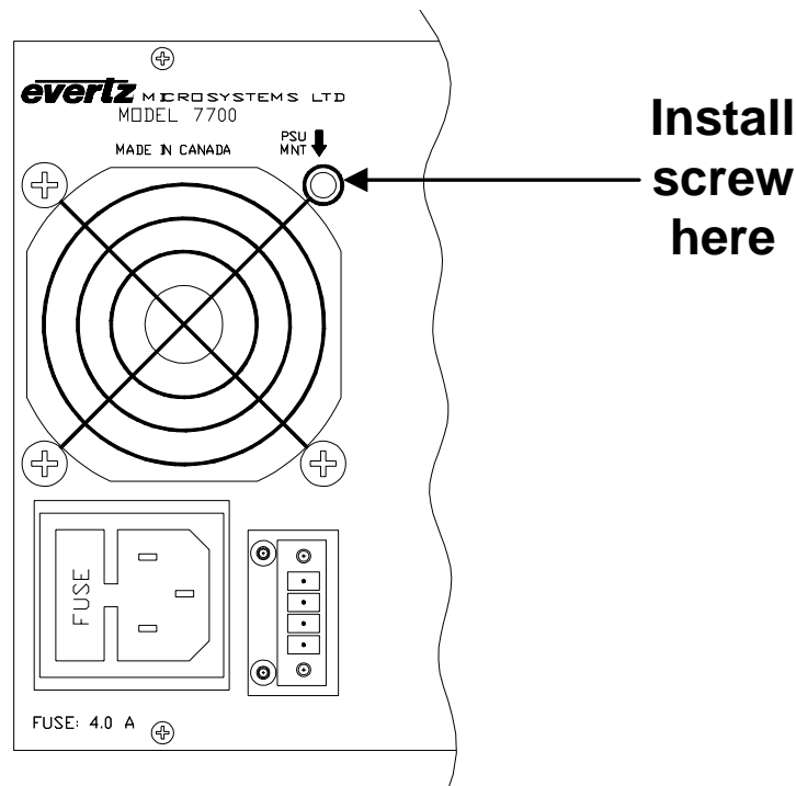
Figure 4-1: Locating the Power Supply Mounting Screw
