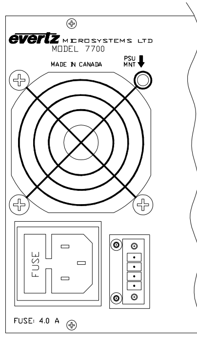
Figure 1-1: 7700FR-C and 7700FR Rear Panel
