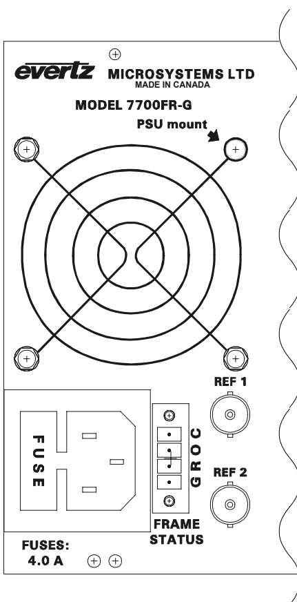
Figure 4: 7700FR-G and 7700FR-D Rear Panel
