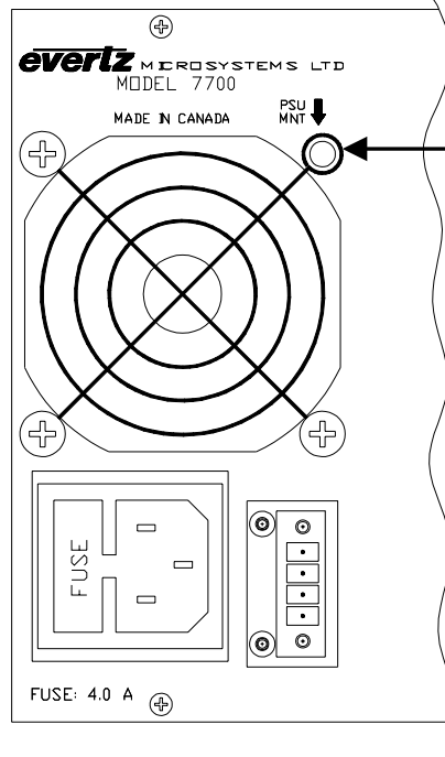
Figure 5: Locating the Power Supply Mounting Screw
