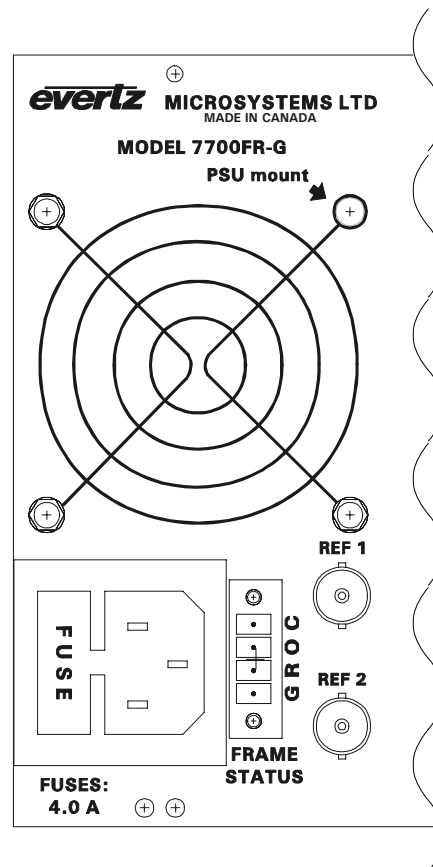
Figure 4-1: 7700FR-G and 7700FR-D Rear Panel
