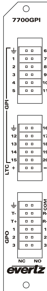
Figure 2-1: 7700GPI Rear Panel
