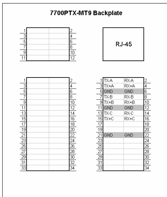
Figure 4-7: RS-422 Pins
