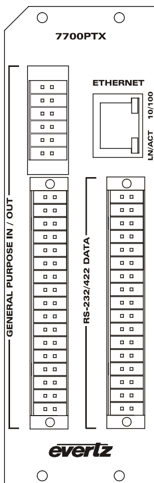
Figure 4-5: 7700PTX Rear Plate
