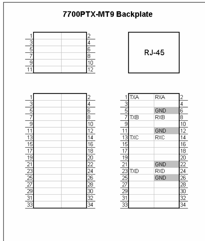
Figure 4-6: RS-232 Pins
