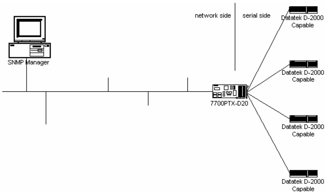
Figure 1-1: Typical 7700PTX-D20 Setup
