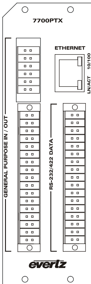
Figure 3-4: 7700PTX Back Plate
