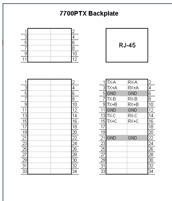
Figure 3-6: RS-422 Pins
