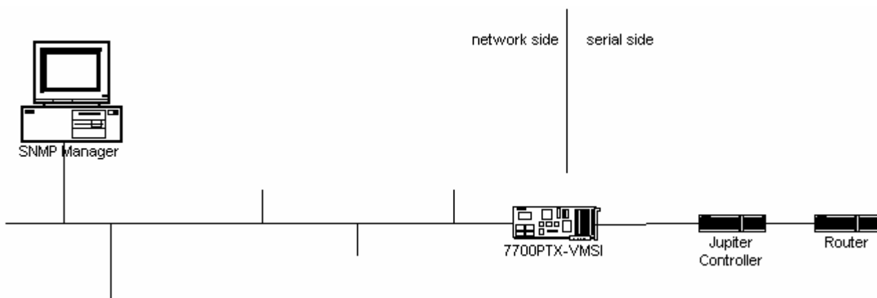
Figure 1-2: Typical 7700PTX-VMSI Setup
