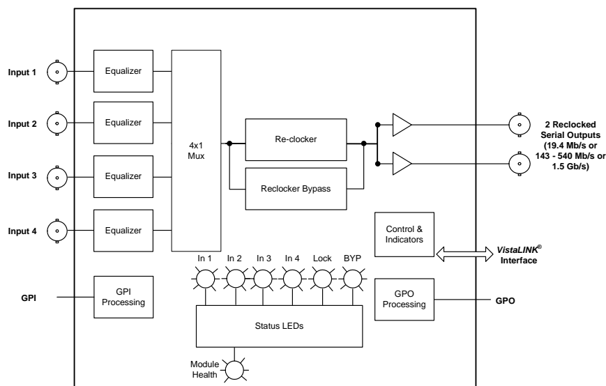
Figure 1-1: 7700R4X1-HD Block Diagram
