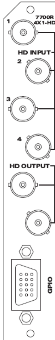
Figure 2-1: 7700R4X1-HD Series Rear IO Module
