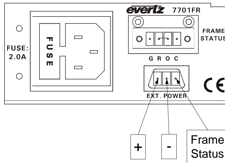
Figure 1: Locating the External Power Connector
