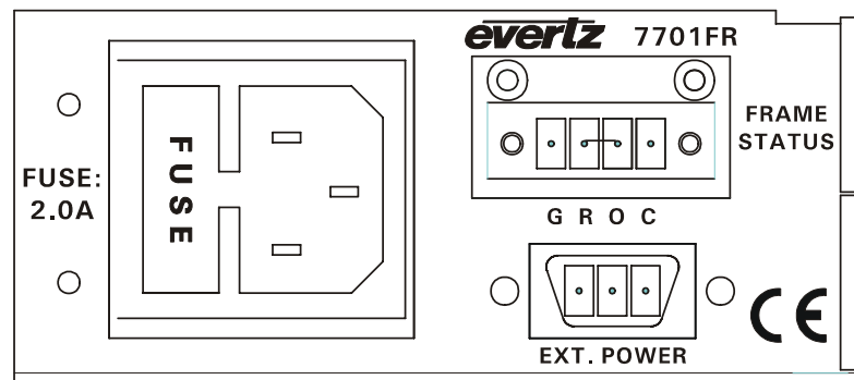
Figure 1: Locating the External Power Connector
