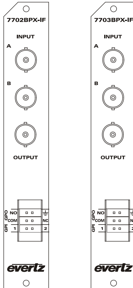
Figure 2-1: 7702BPX-IF and 7703BPX-IF Rear Panels
