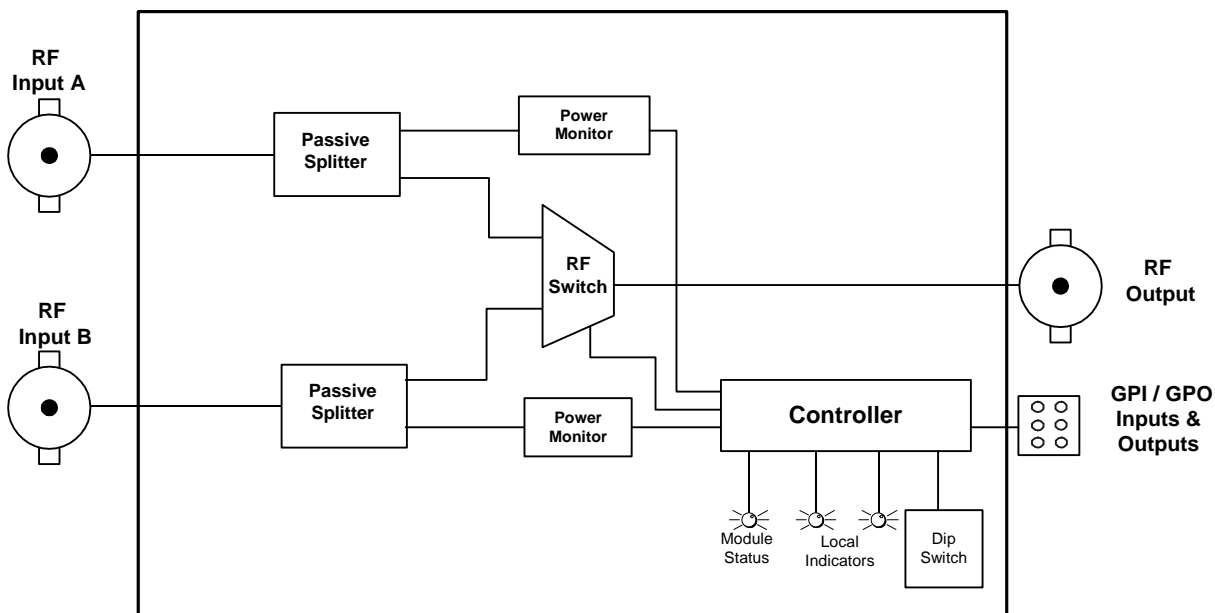
Figure 1-2: 7702BPX-IF Block Diagram
