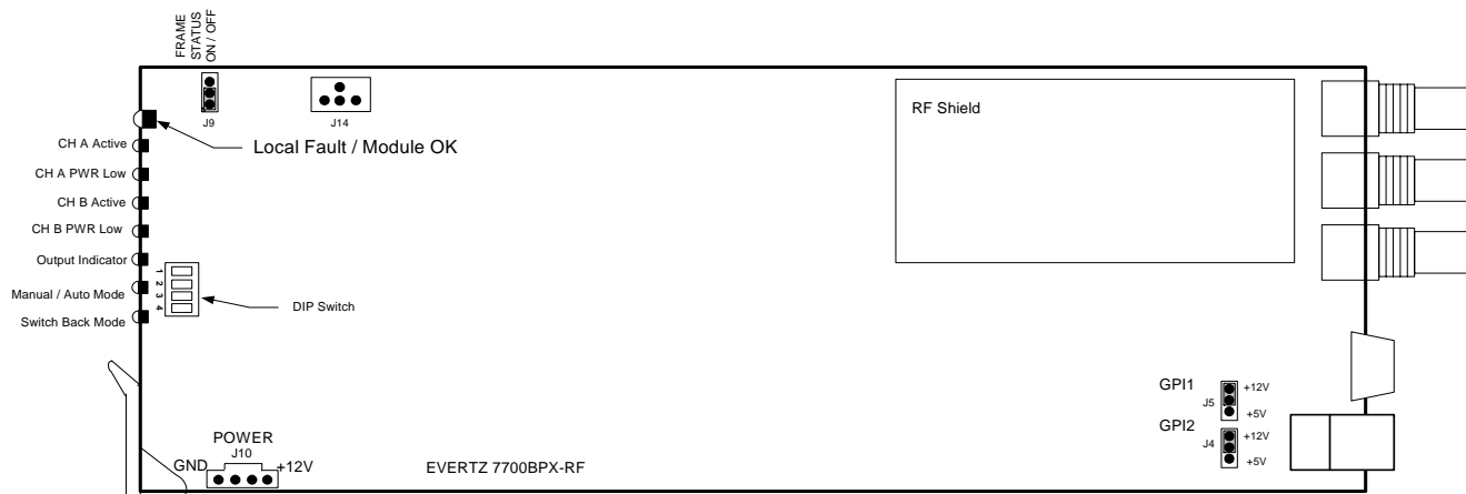
Figure 6-1: Location of Jumpers – 7702BPX-IF
