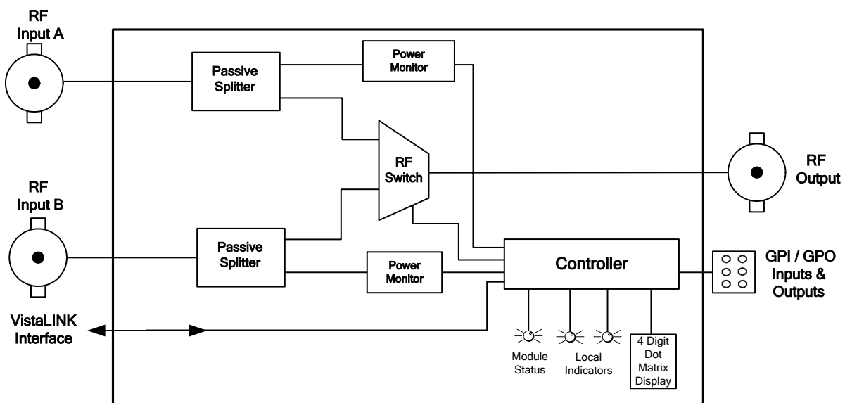
Figure 1-1: 7703BPX-IF Block Diagram
