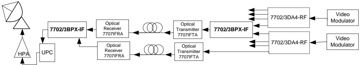
Figure 1-3: Typical Application of Protection Switch in IF Uplink Transport System
