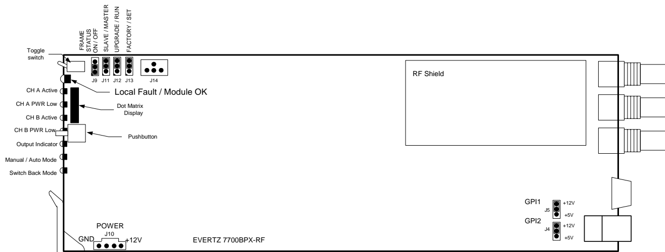
Figure 6-2: Location of Jumpers – 7703BPX-IF
