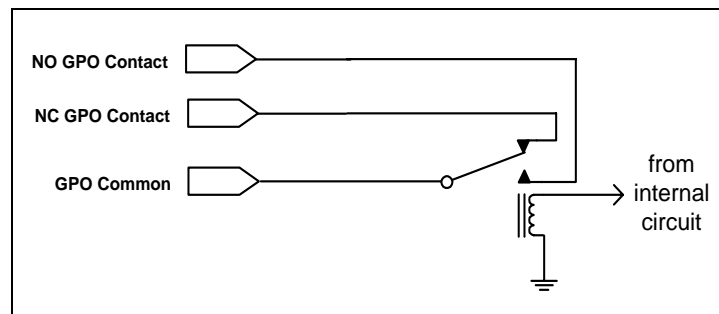
Figure 2-3: GPO Configuration
