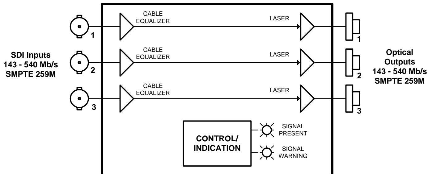
Figure 1-1: 7705EO-3 Block Diagram
