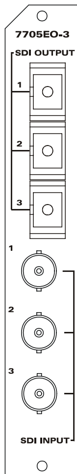
Figure 2-1: 7705EO-3 Rear Panel
