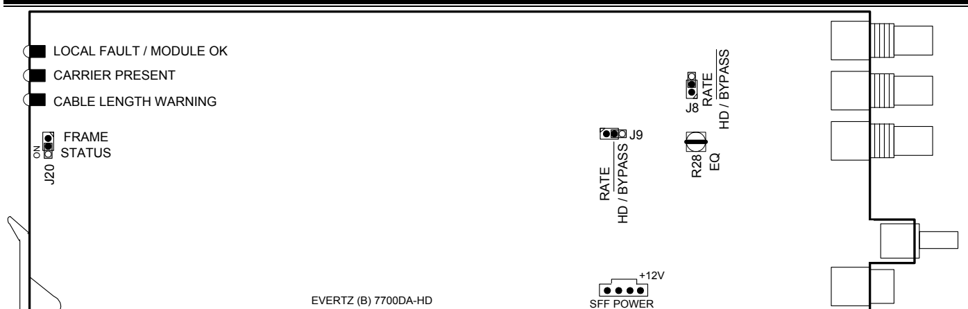
Figure 5: Jumper Locations for Rev B DA Cards
