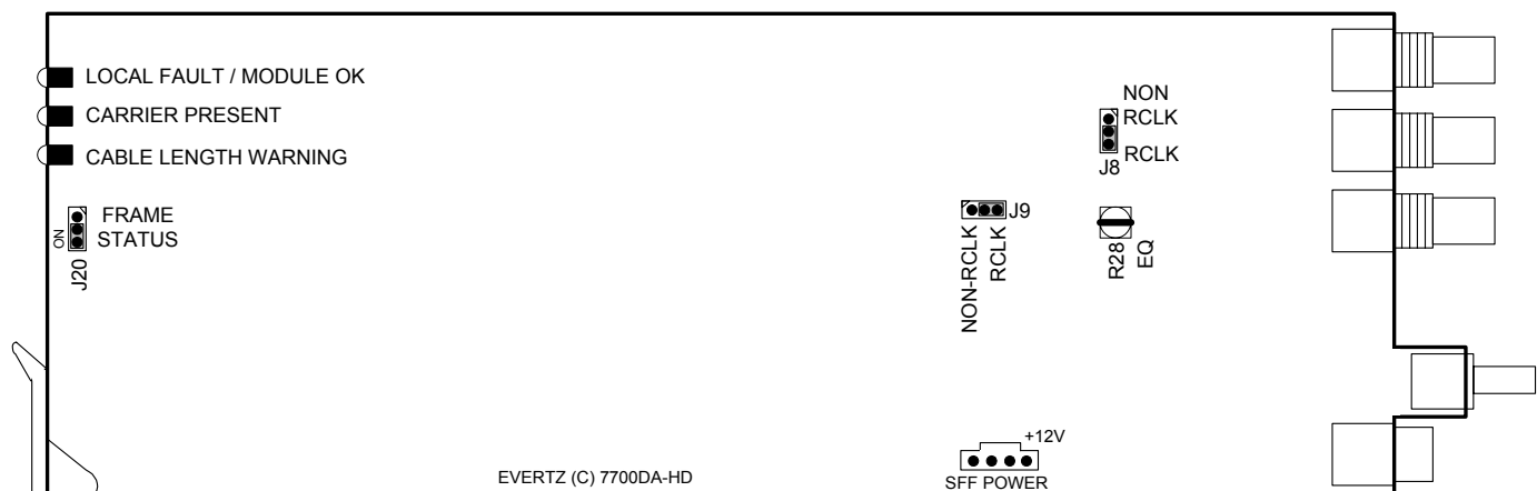
Figure 6: Jumper Locations for Rev C DA Cards
