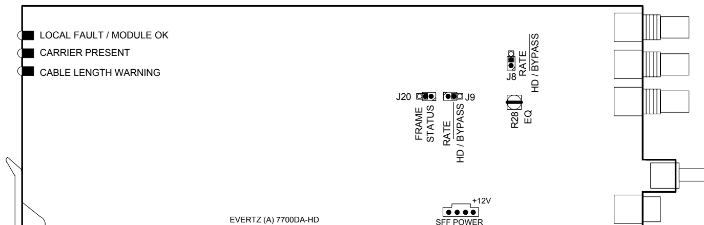
Figure 4: Jumper Locations for Rev A and Rev 1 DA Cards
