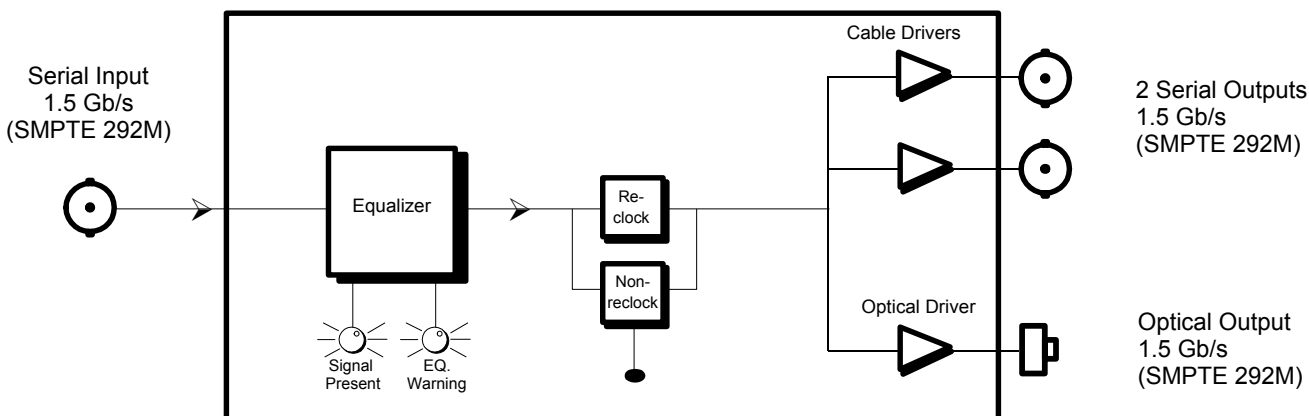
Figure 1: 7705EO-HD Block Diagram
