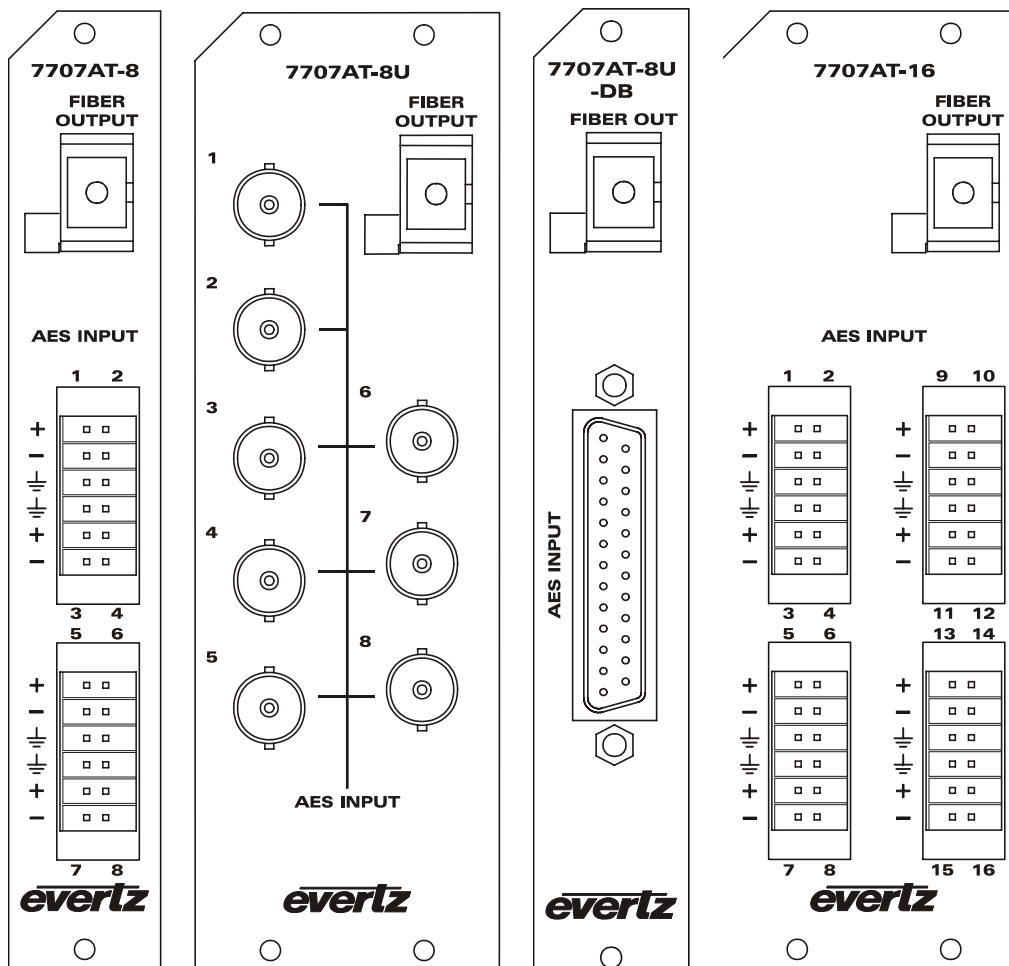
Figure 2-1: 7707AT Rear Panels
