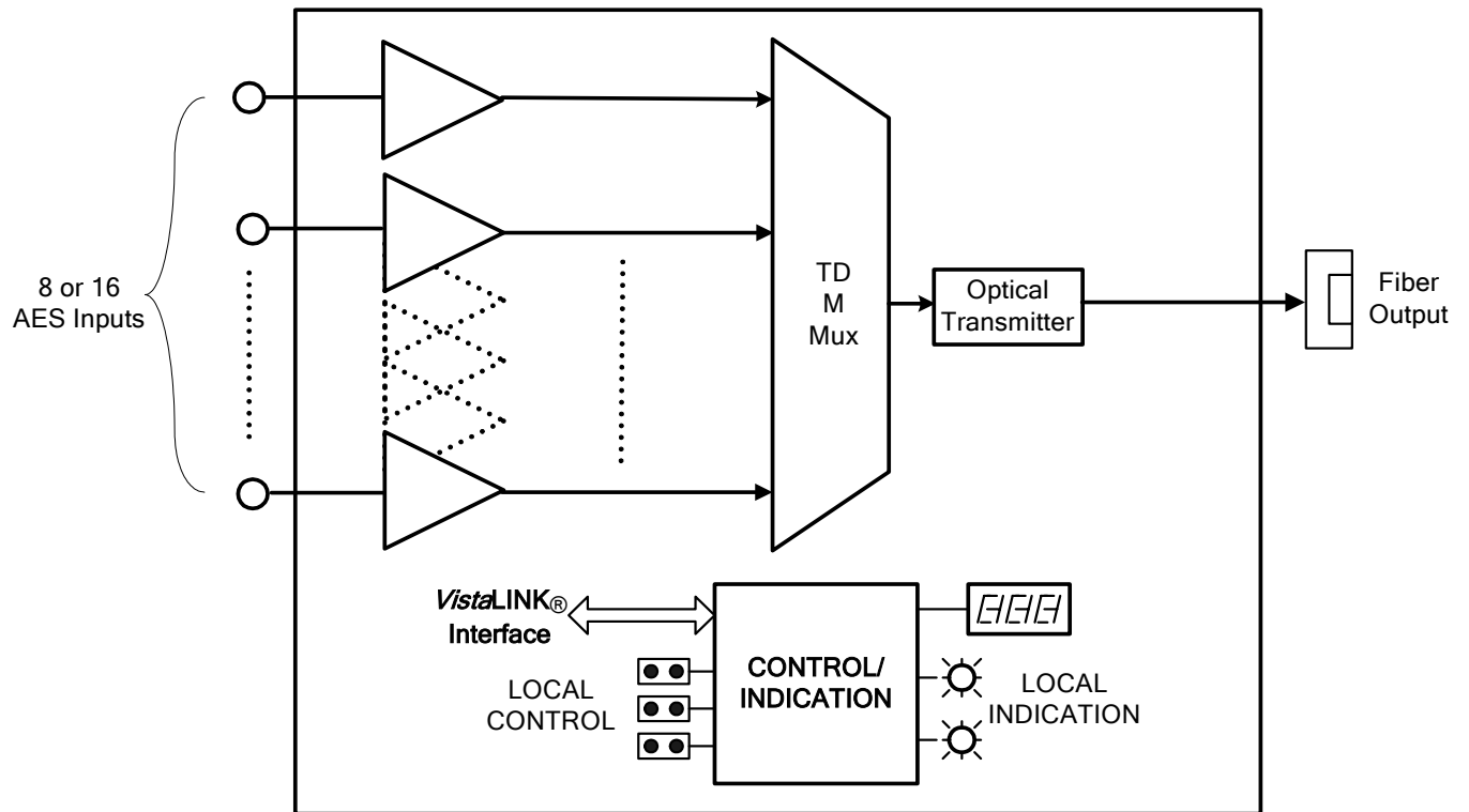
Figure 1-1: 7707AT Block Diagram
