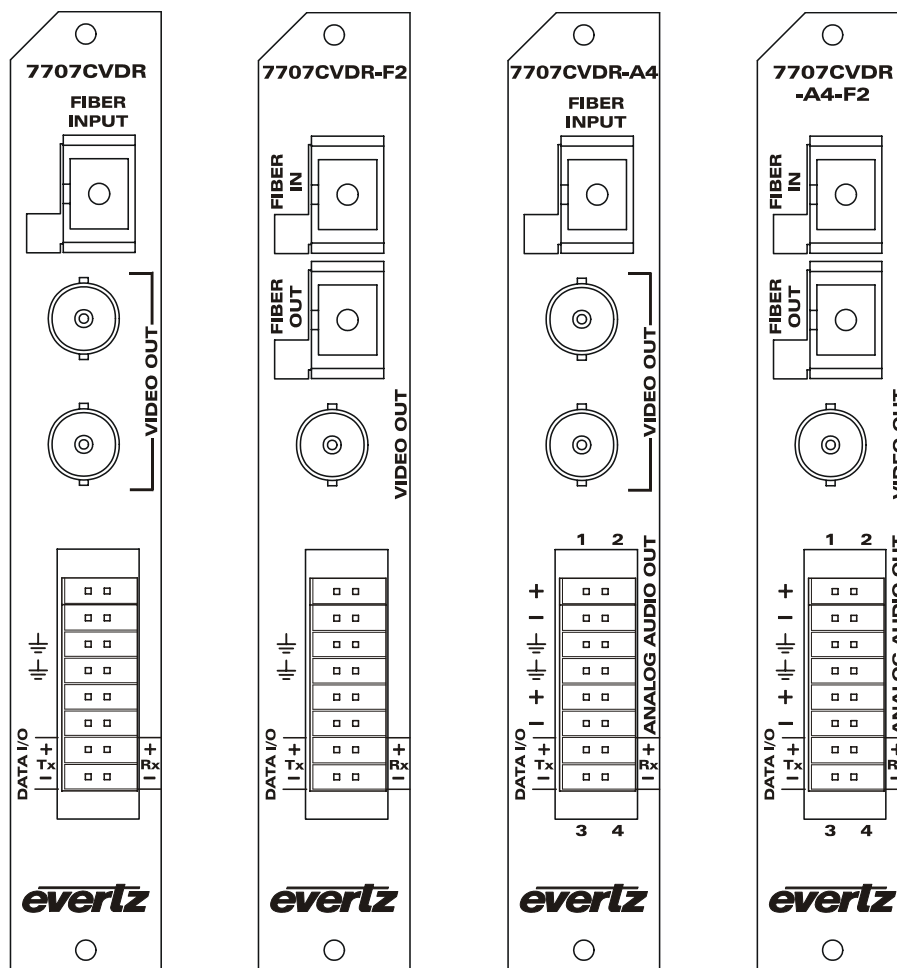
Figure 2-1: 7707CVDR and 7707CVDR-A4 Rear Panels
