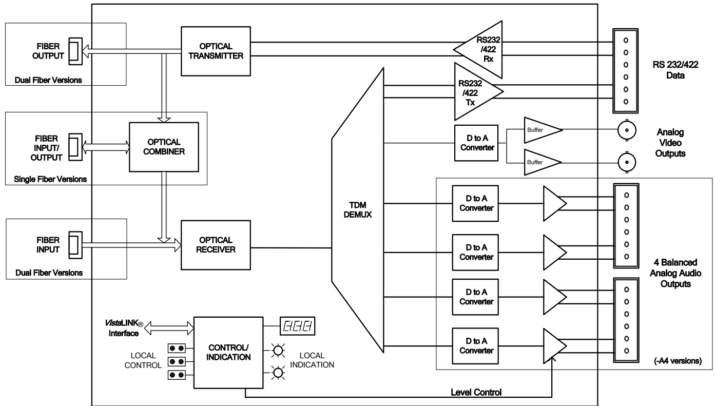
Figure 1-1: 7707CVDR Block Diagram
