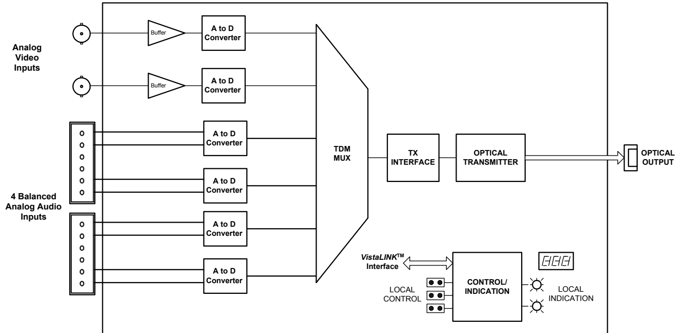
Figure 2: 7707CVT-2 Block Diagram
