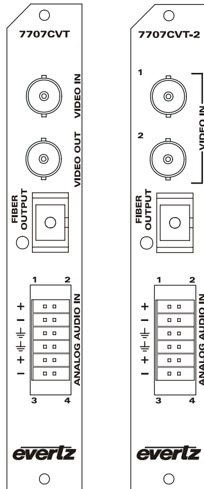
Figure 4: 7707CVT Rear Panels
