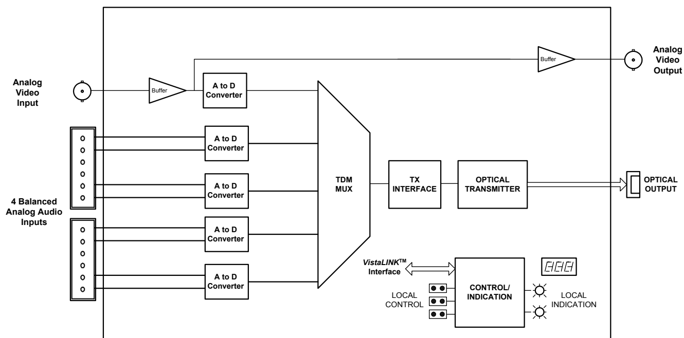
Figure 1: 7707CVT Block Diagram
